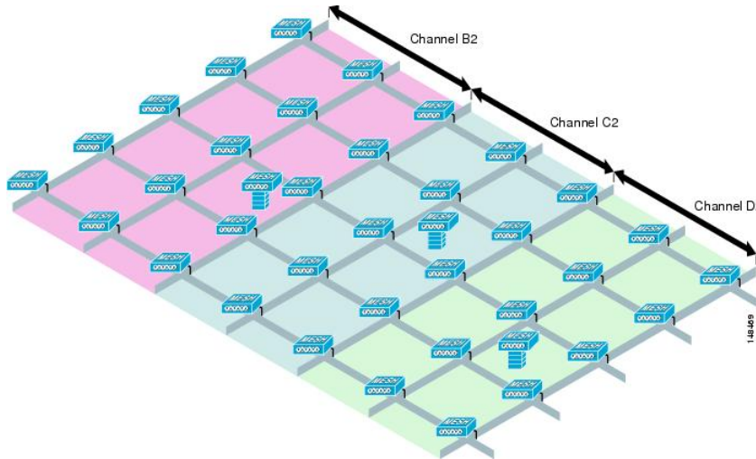
Figure 29: Multiple RAP and MAP Cells
