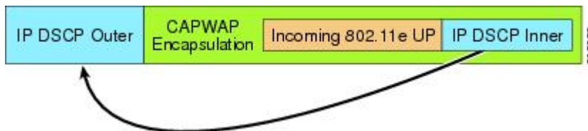
Figure 62: MAP to RAP Path
