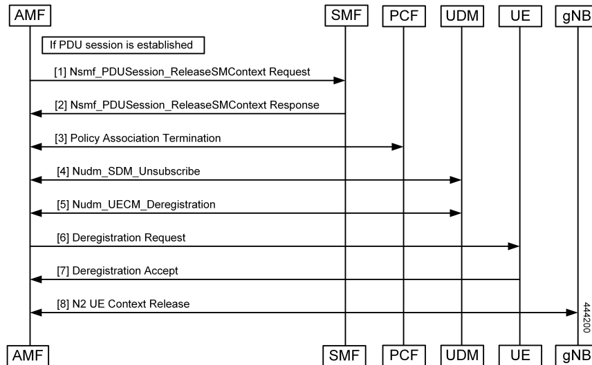
Figure 31: AMF-Initiated Deregistration Call Flow
