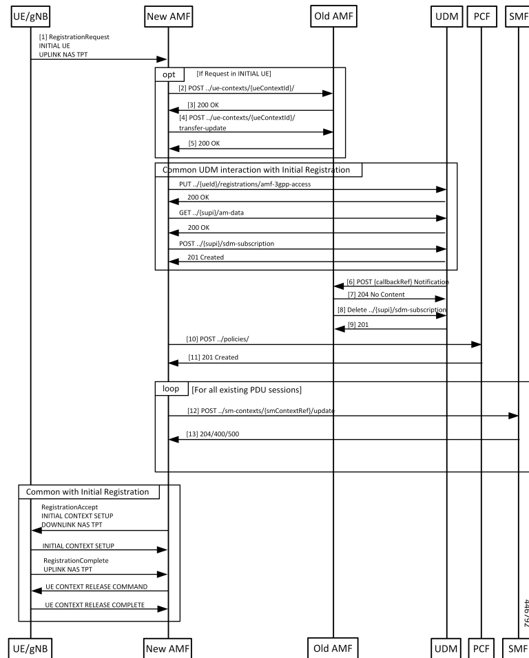
Figure 42: Registration with AMF Change Call Flow
