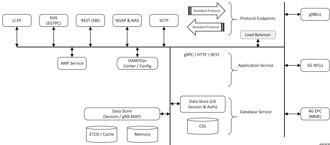
Figure 7: AMF Architecture
