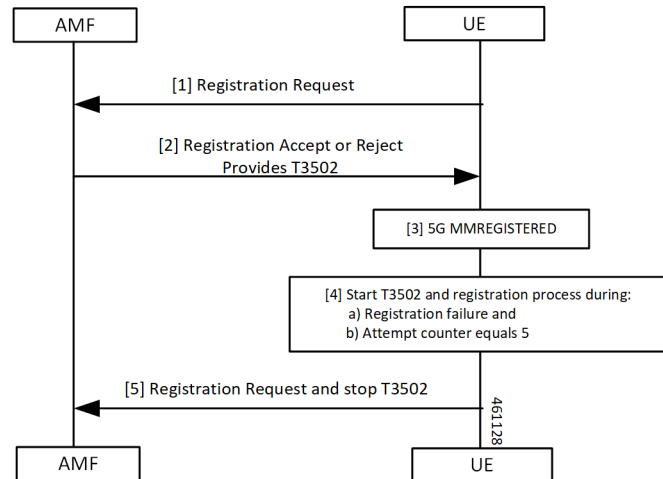
Figure 58: T3502 Timer Call Flow
