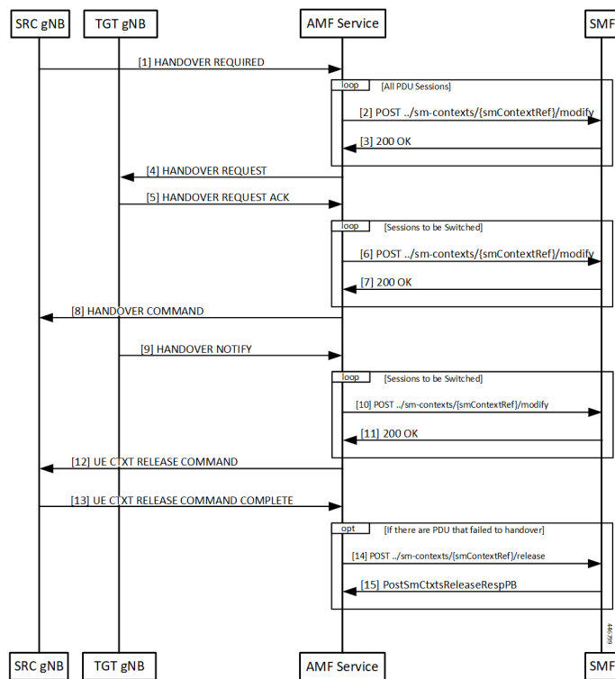
Figure 45: N2 Handover without AMF Change Call Flow
