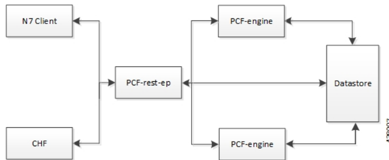
Figure 20: N28 Interface
