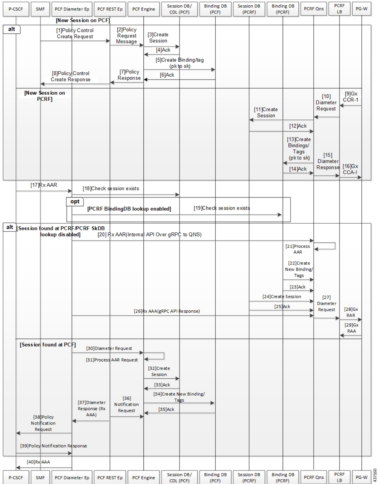
Figure 44: Session Creation, Update, and Termination Call Flow
