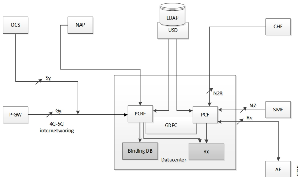
Figure 6: PCF Deployment
