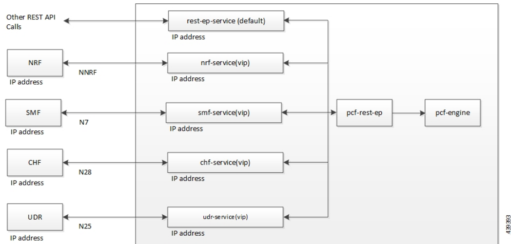
Figure 19: Multiple VIPs
