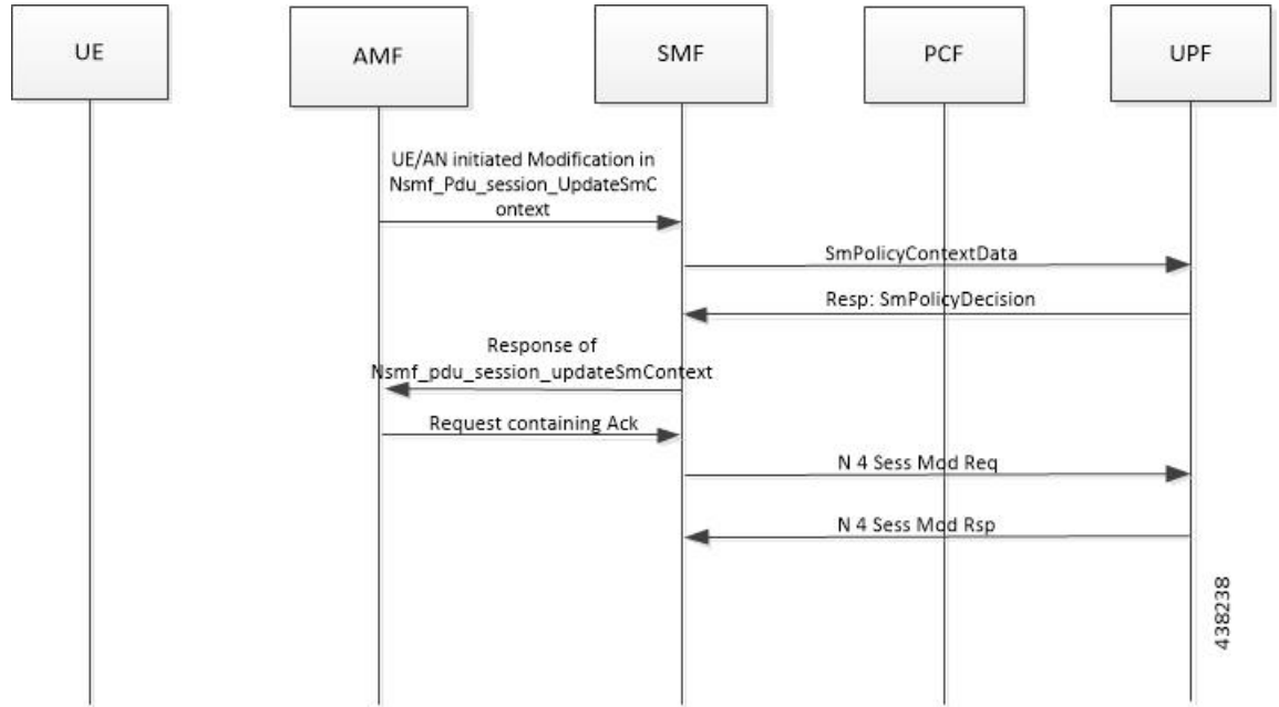
Figure 104: UE/AN-initiated Modify
