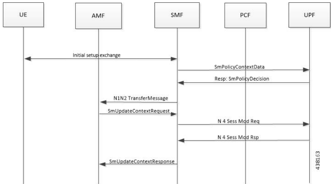
Figure 103: Setup Creation
