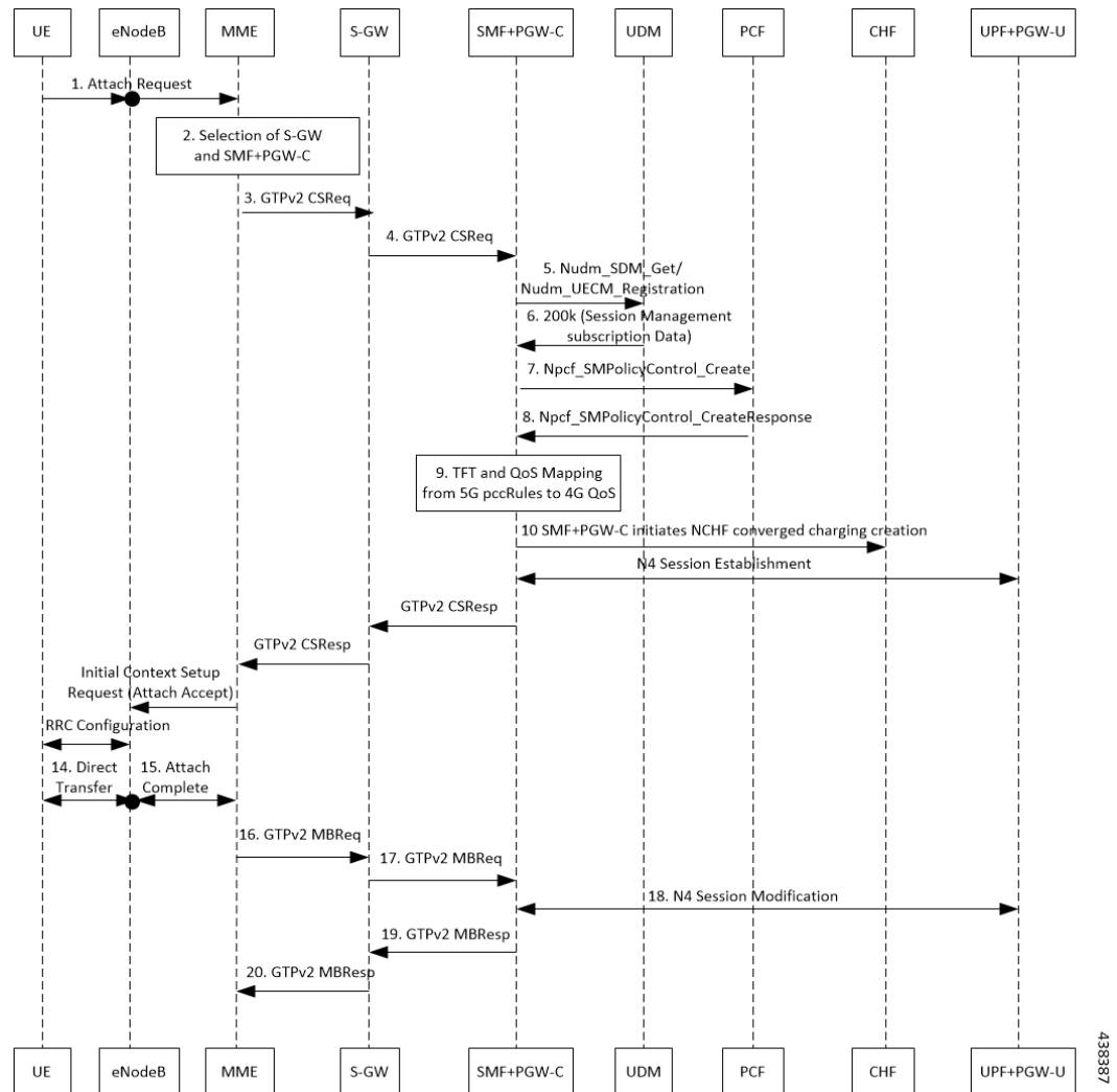
Figure 125: VoLTE PDU Session Creation Call Flow
