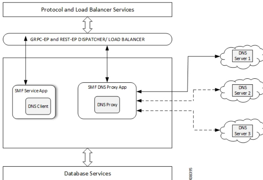
Figure 28: DNS Proxy Feature Integration in SMF
