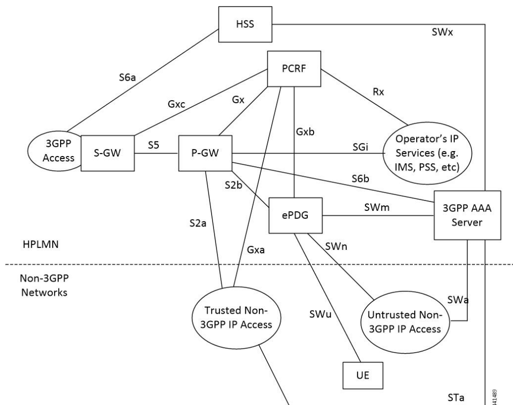
Figure 133: Non-Roaming Architecture Within EPS using S5, S2a, and S2b Interfaces
