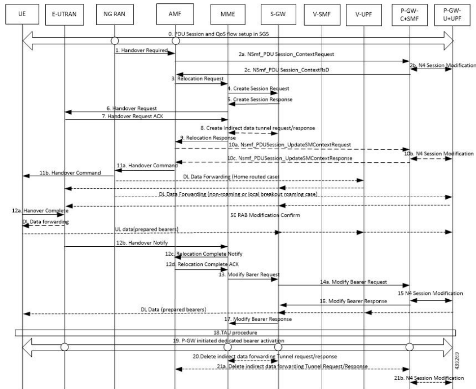
Figure 42: 5G to EPS Handover with IDFT Timer Call Flow
