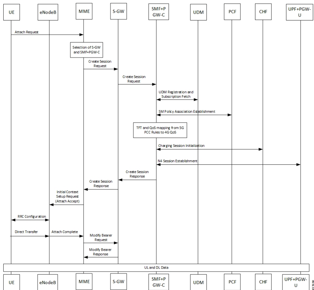
Figure 31: Call Flow for Initial Attach on E-UTRAN via 5G Core
