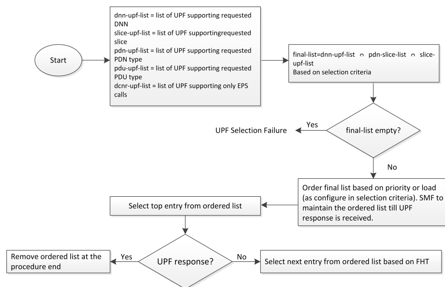
Figure 107: UPF Node Selection Workflow
