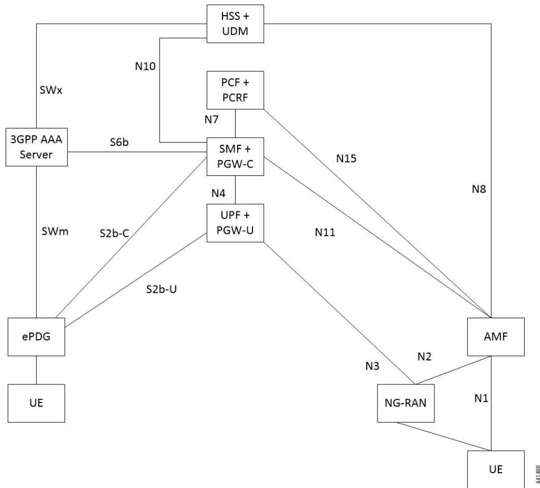
Figure 132: Non-Roaming Architecture for Interworking between ePDG or EPC and 5GS
