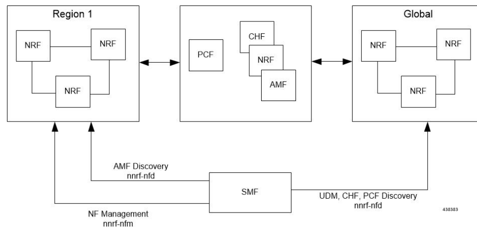
Figure 94: NRF Deployment
