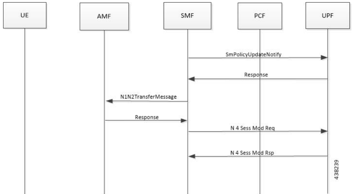
Figure 105: UDM/PCF-initiated Modify
