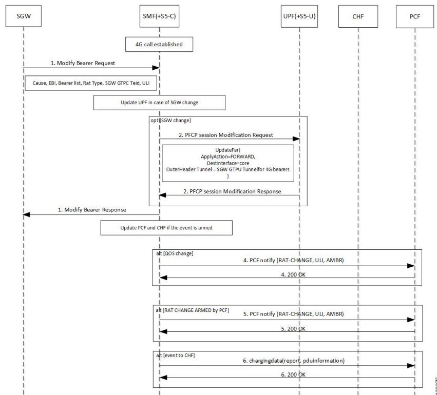
Figure 45: X2 and S1 based Handover for EPS Session Connected to SMF
