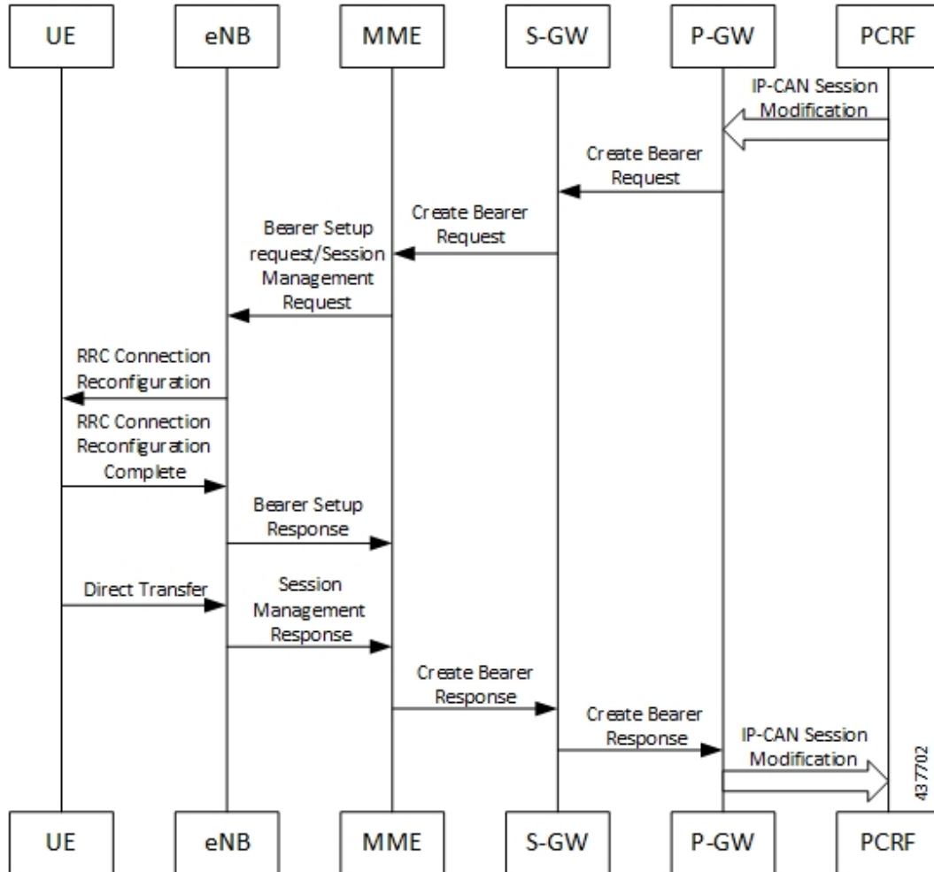
Figure 35: Dedicated Bearer Creation Call Flow
