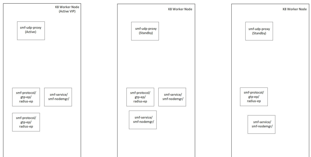
Figure 117: UDP Proxy Architecture
