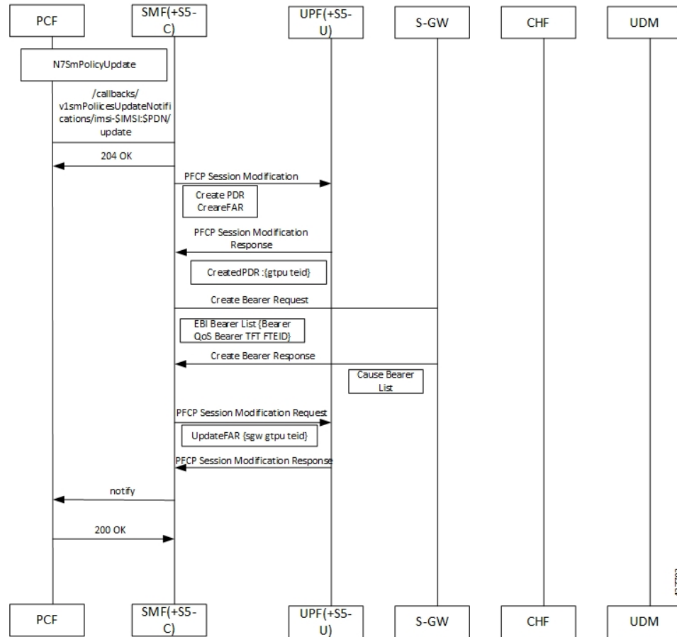
Figure 36: PCF-initiated Dedicated Bearer Activation
