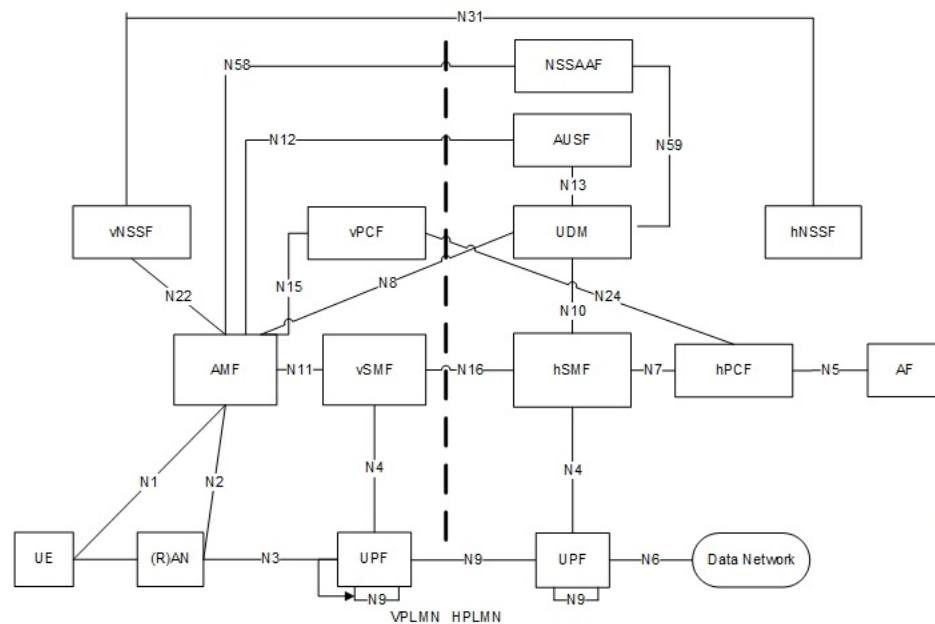
Figure 205: 5G NR HR Roaming Architecture
