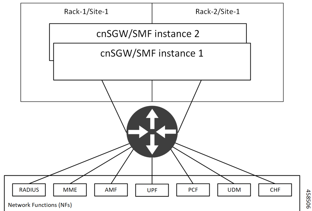
Figure 198: Active-Active GR Deployment
