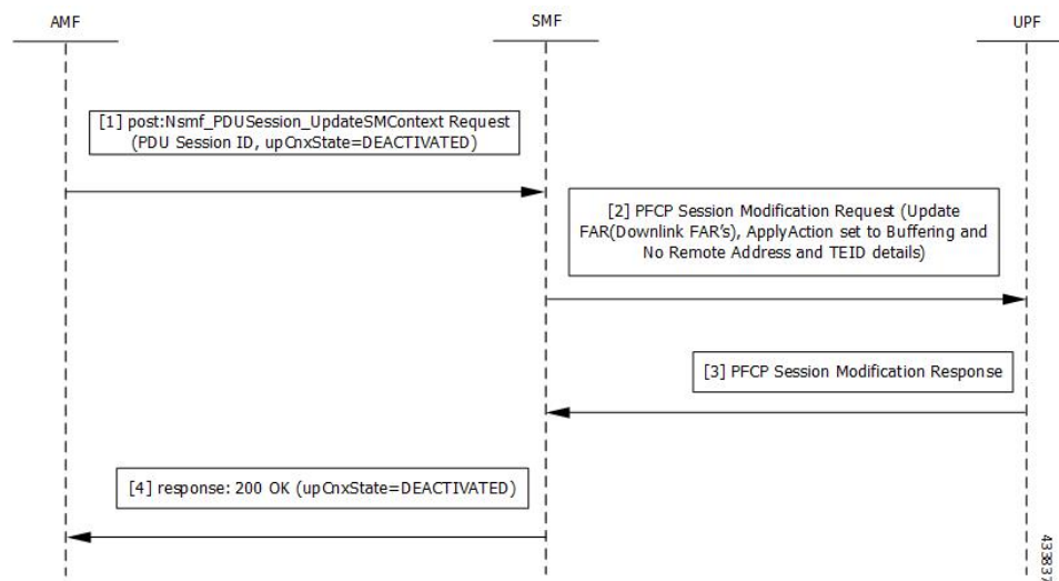
Figure 236: Deactivation of the User Plane Connection Call Flow
