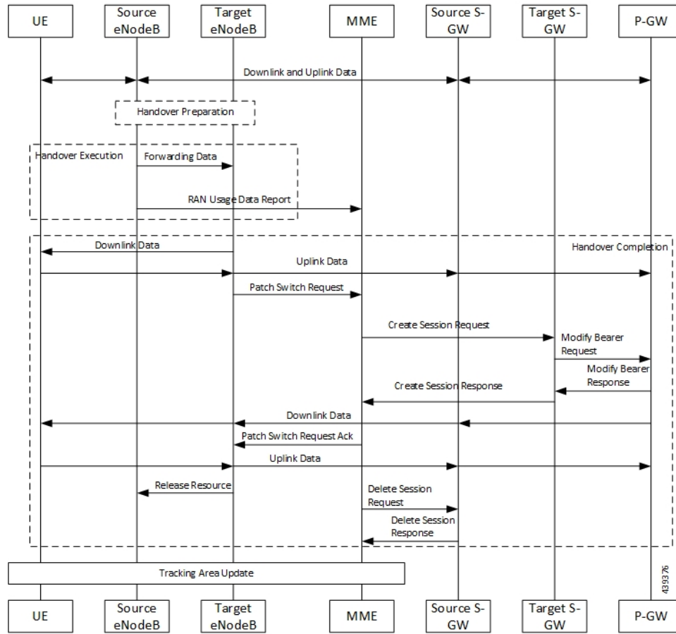
Figure 52: X2-Based Handover with SGW Relocation Call Flow
