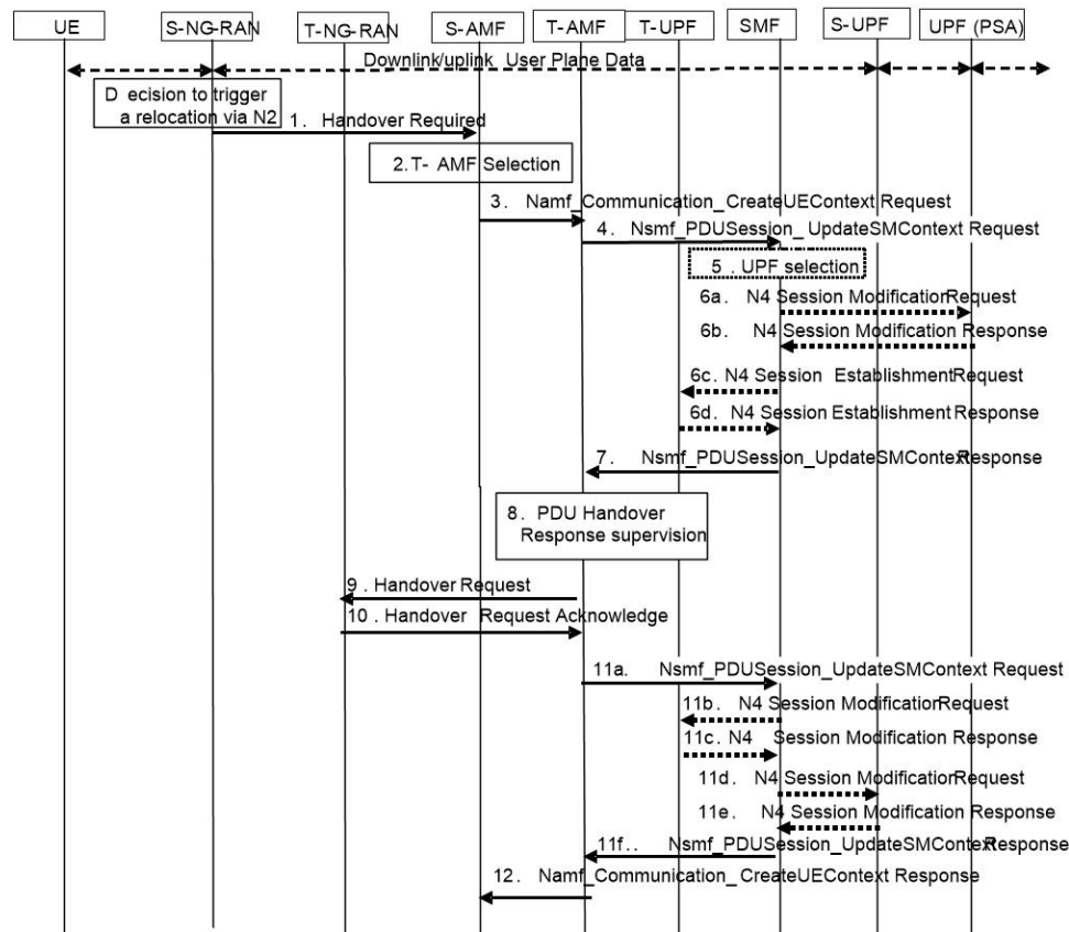
Figure 98: Inter NG-RAN Node N2-based Handover - Preparation Phase
