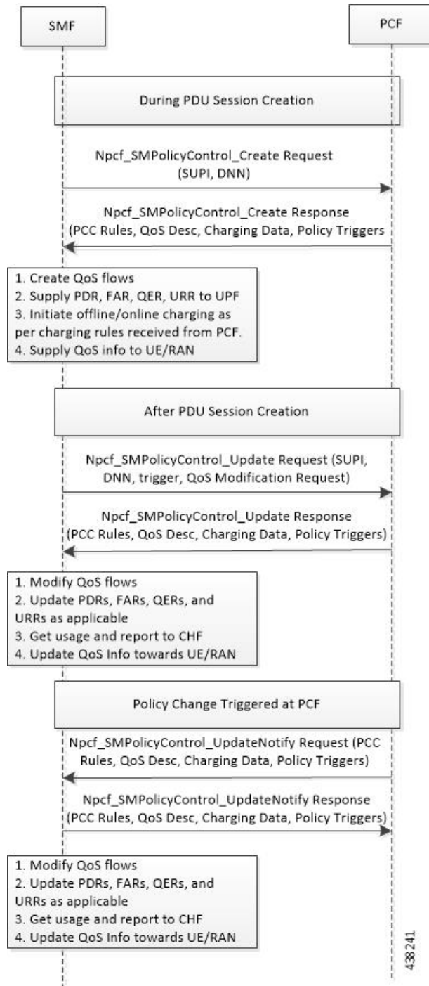
Figure 178: Dynamic Policy Management Call Flow
