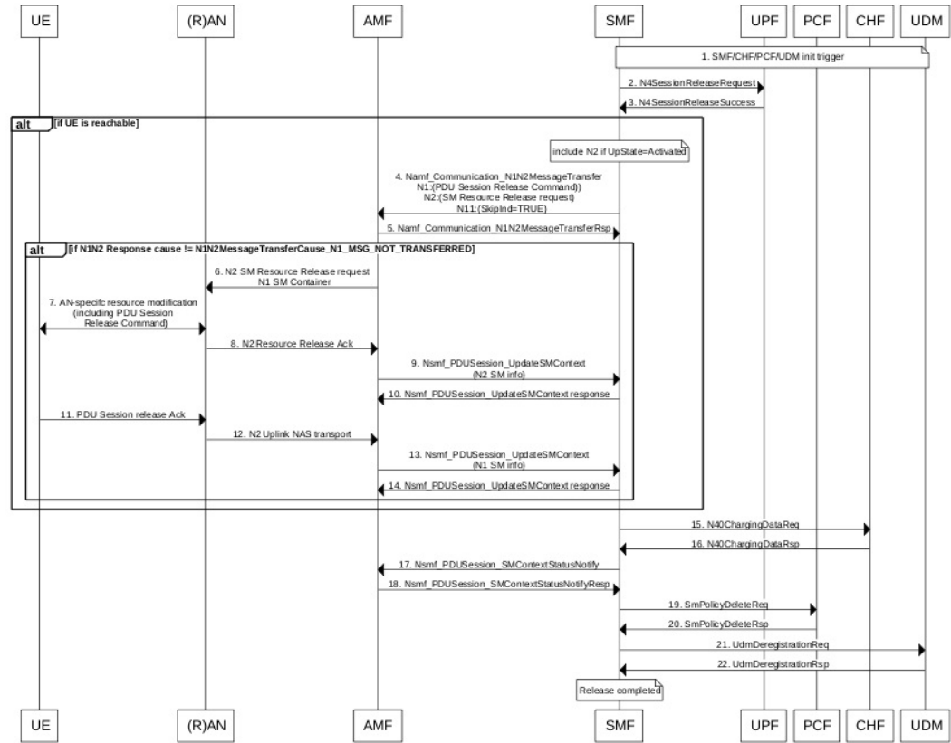
Figure 60: Network-initiated PDU Session Release Call Flow
