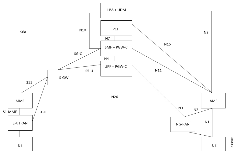
Figure 84: Network Architecture for the EPS-5G Core Interworking
