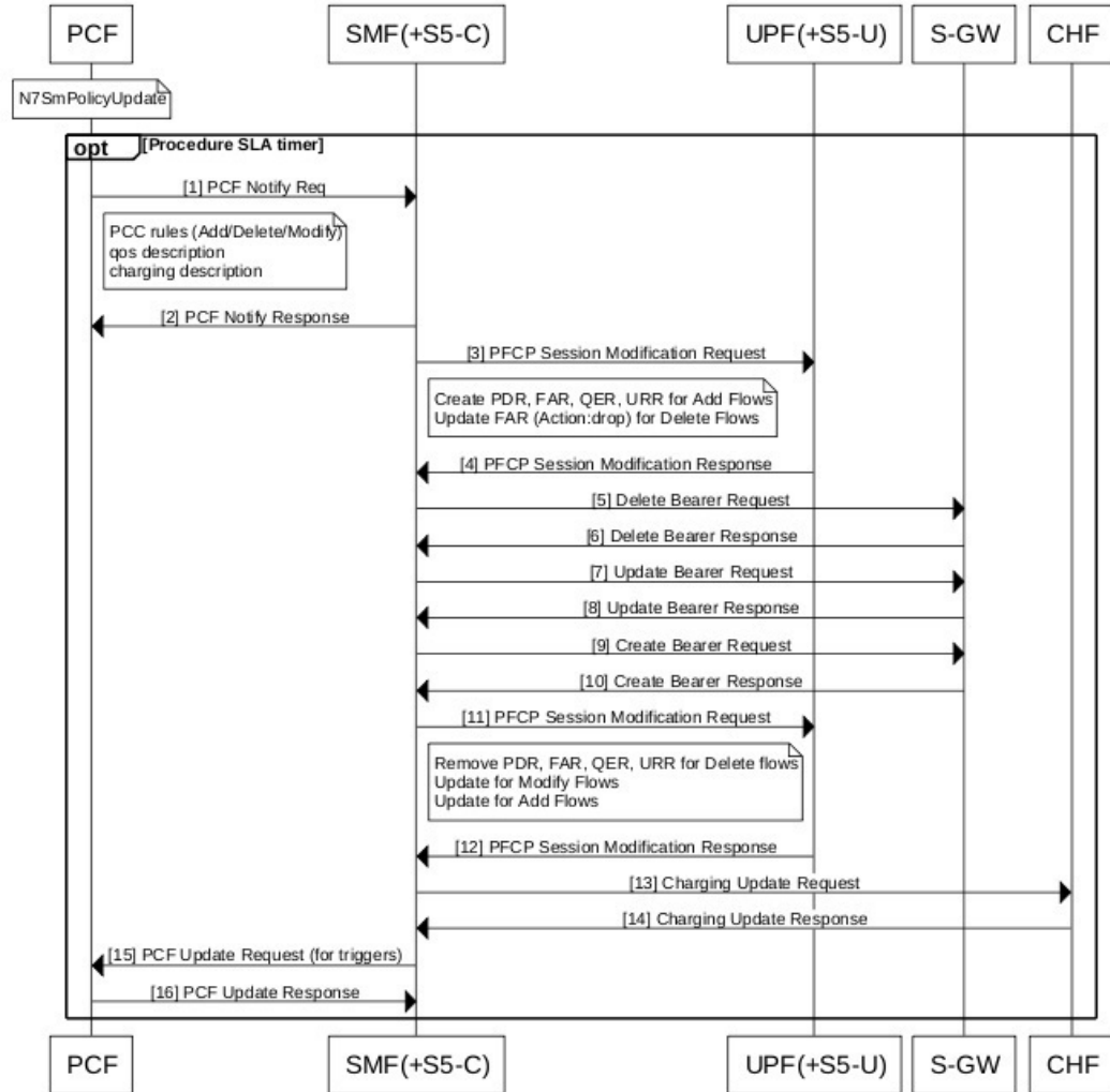
Figure 68: PCF-initiated Modification Call Flow
