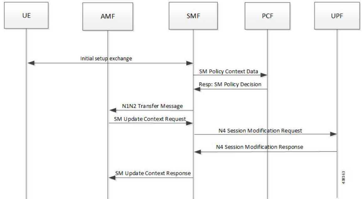
Figure 173: Setup Creation Call Flow
