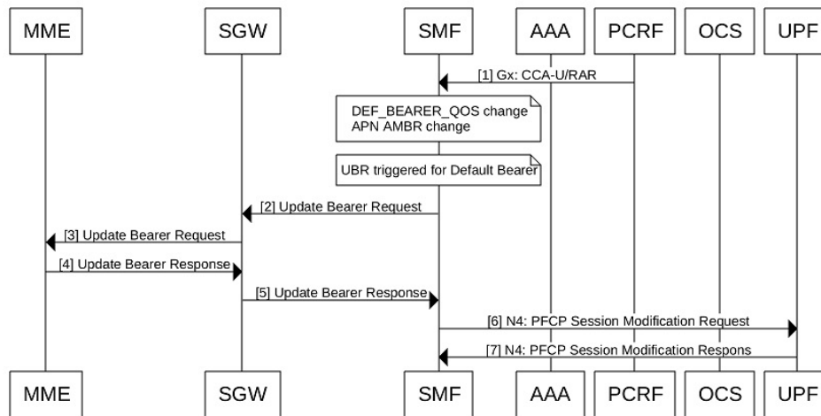
Figure 54: Call Flow for E-UTRAN Network (PCRF) CCAU/RAR Initiated UBR
