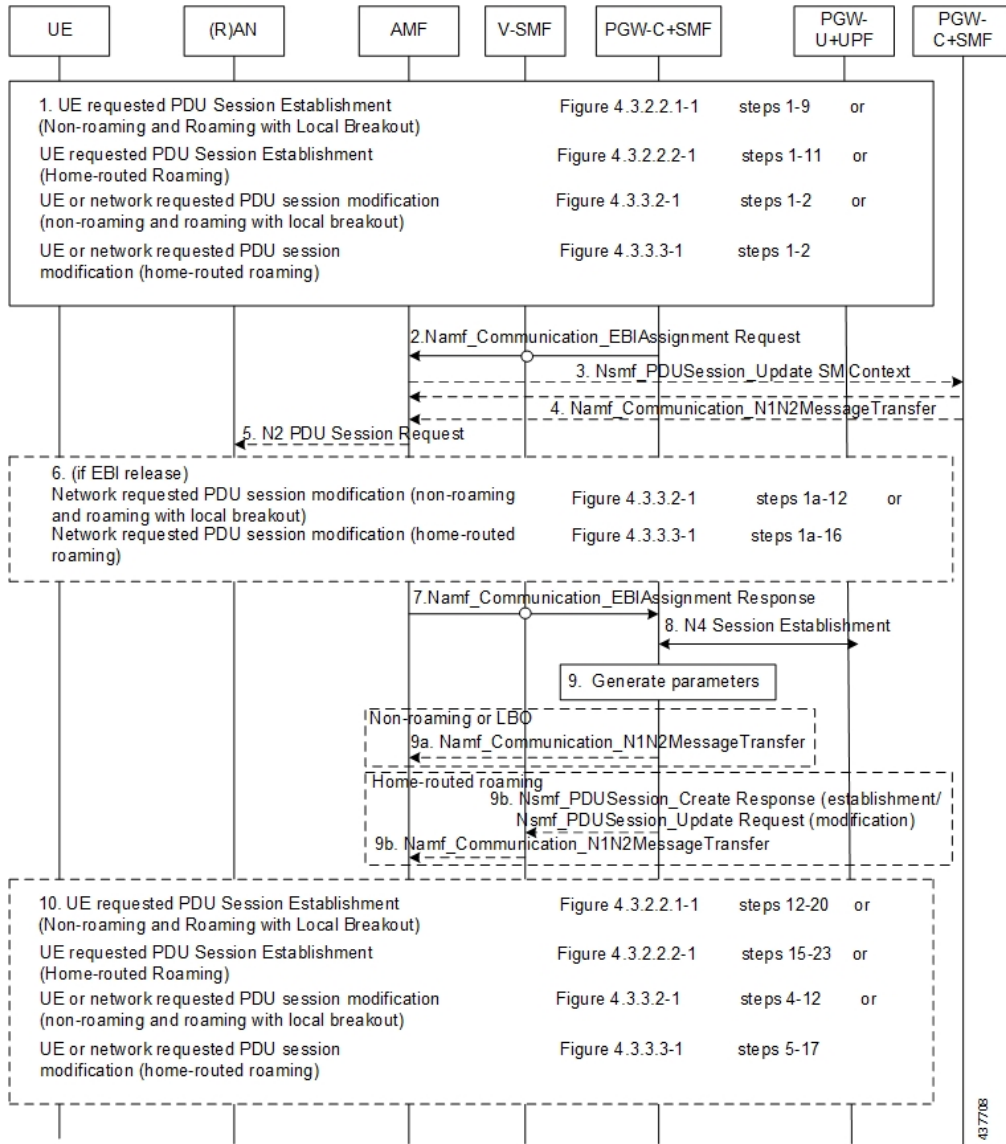
Figure 64: EPS Bearer ID Allocation Call Flow
