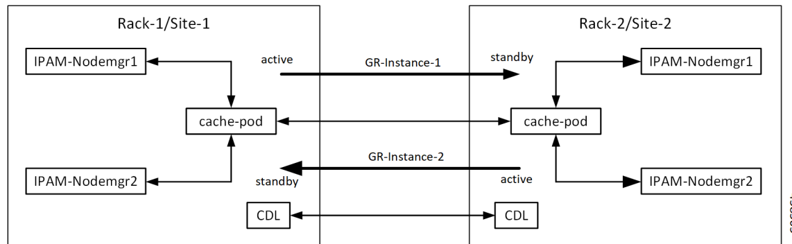
Figure 200: IPAM
