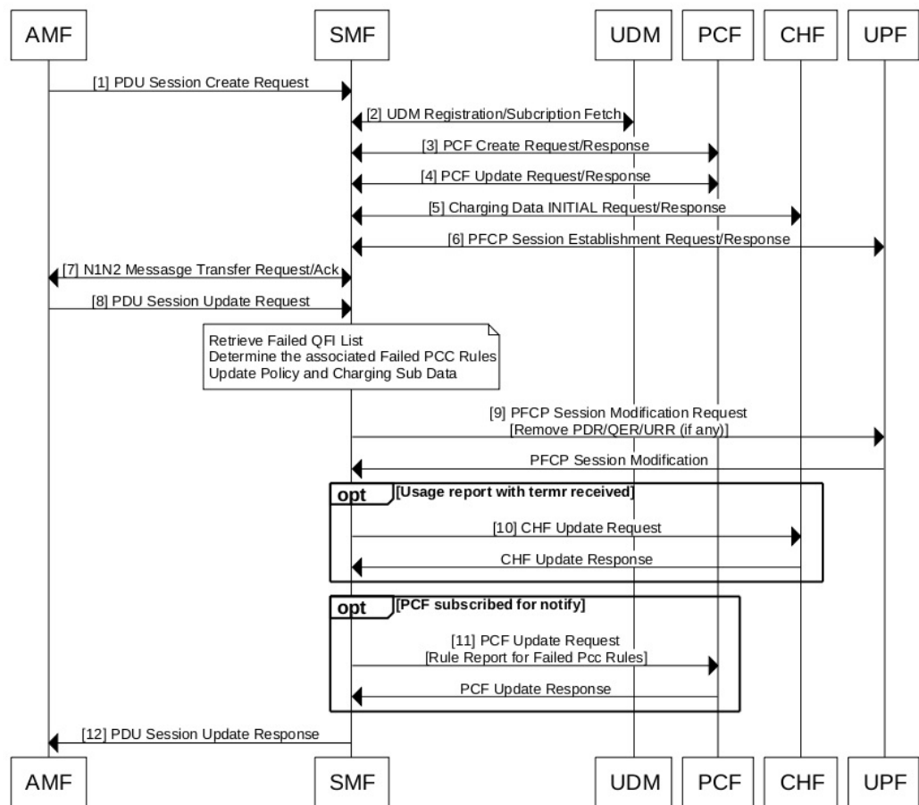
Figure 80: Handling Failed QFIs During PDU Setup
