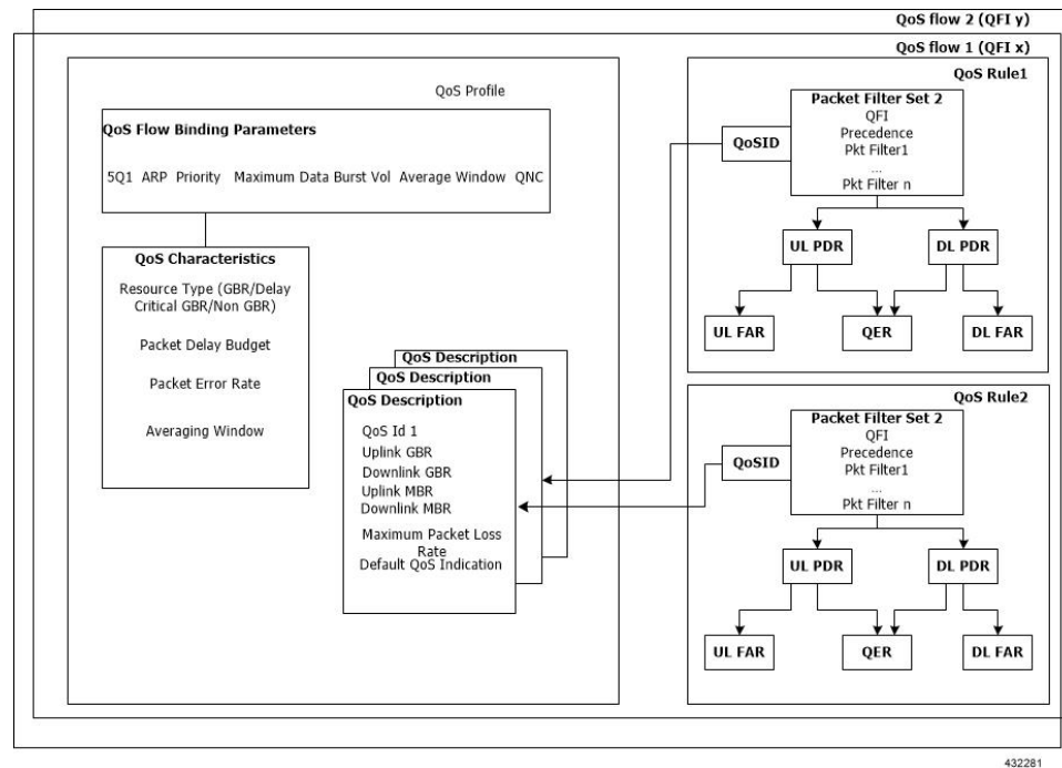
Figure 176: QoS Information Management at SMF
