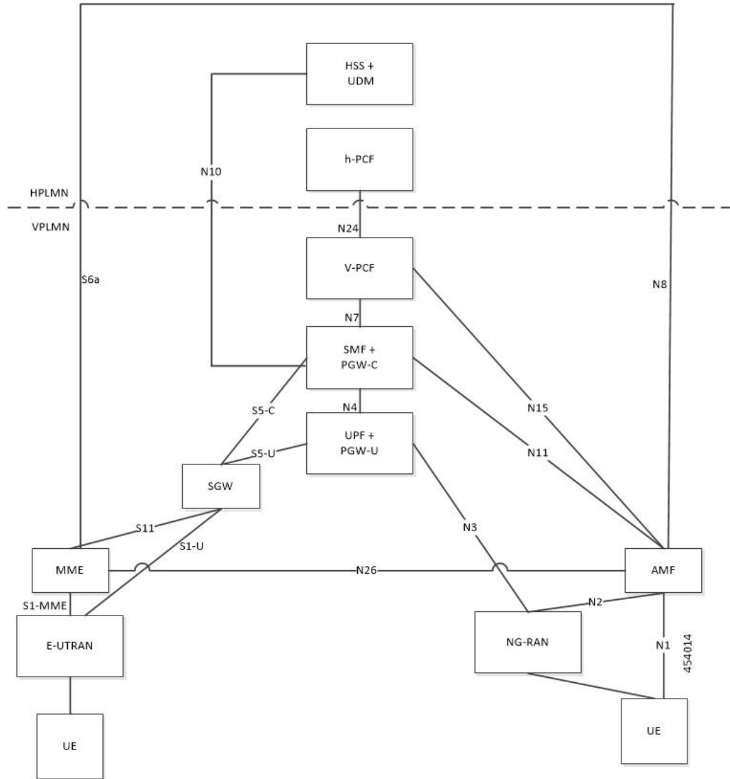
Figure 201: Local Breakout Roaming Architecture for 4G Sessions
