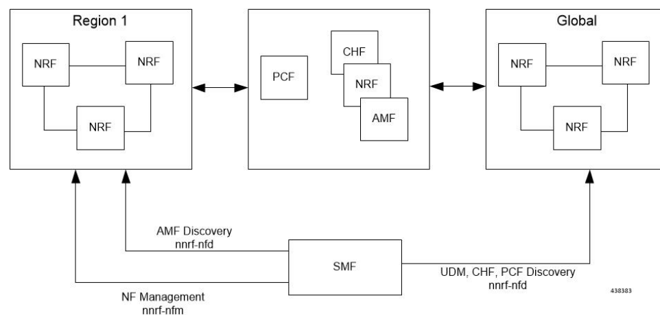
Figure 168: NRF Deployment
