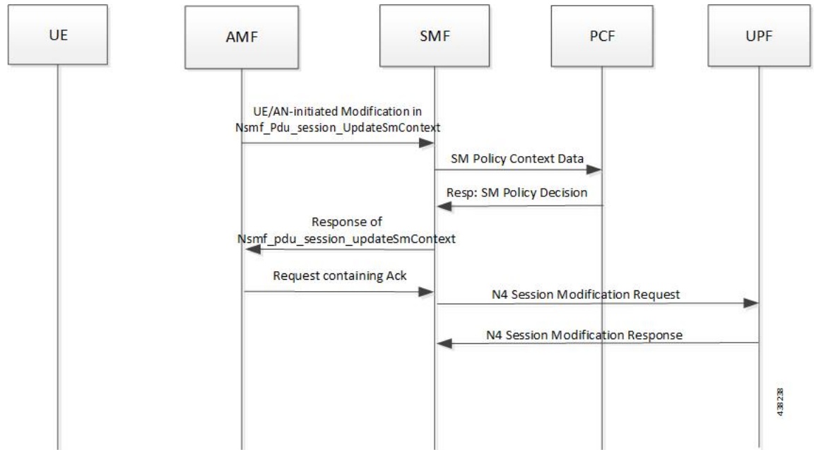
Figure 174: UE/AN-initiated Modification Call Flow
