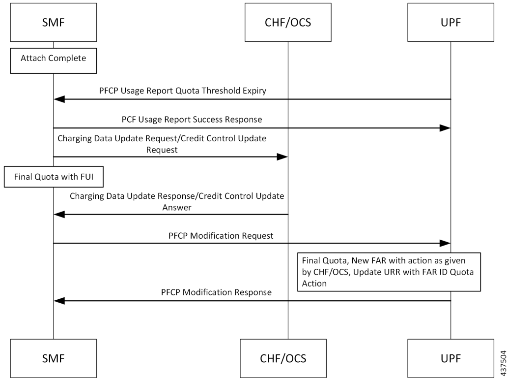
Figure 232: FUI in the Charging Data Initial or Update Response from CHF
