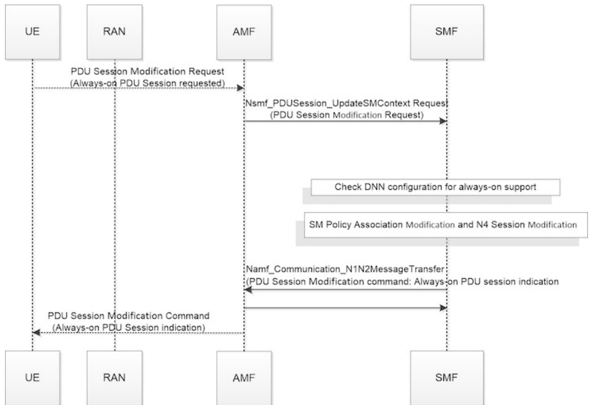
Figure 244: UE-requested PDU Session Modification Call Flow
