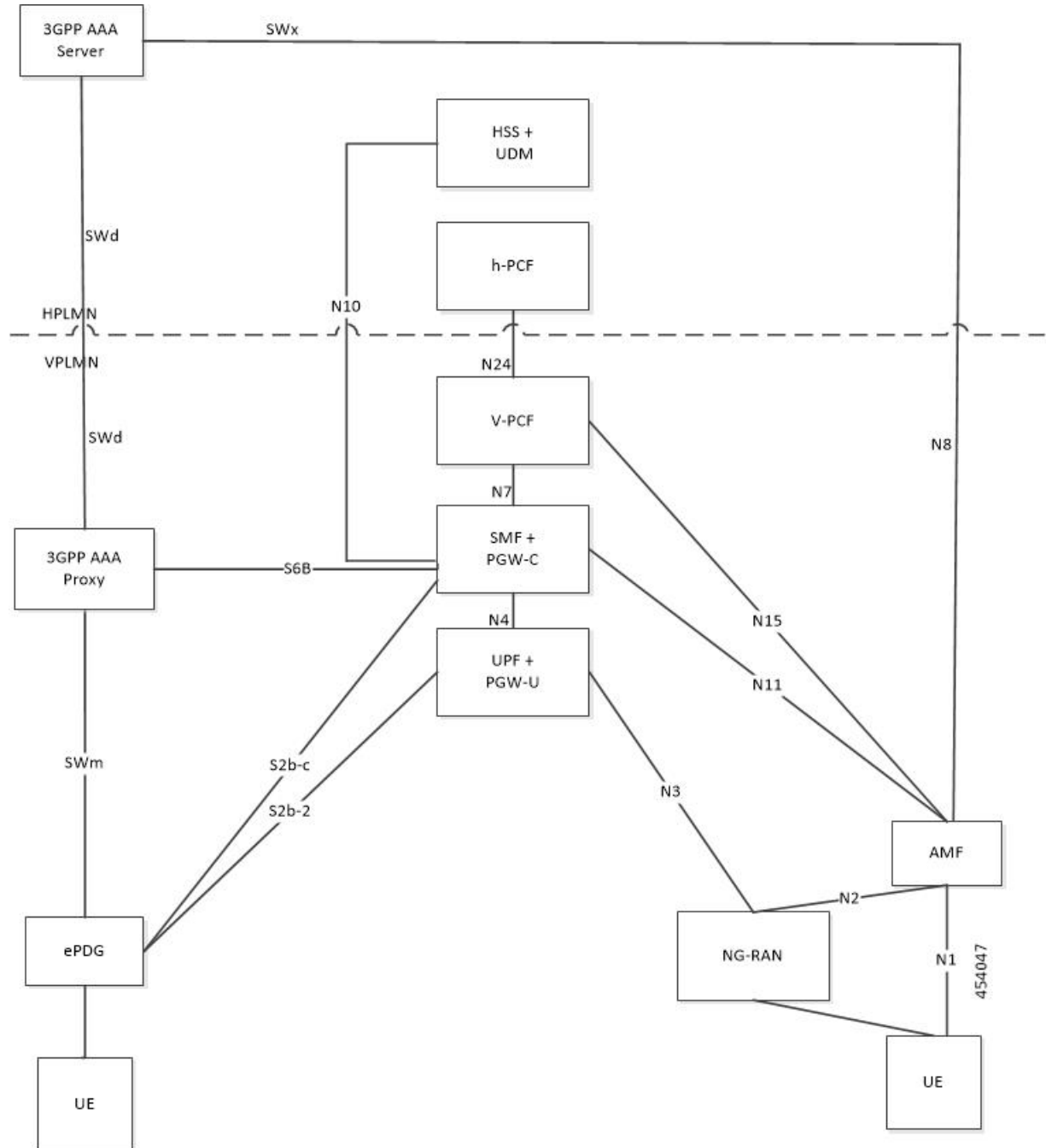
Figure 202: Local Breakout Roaming Architecture for Wi-Fi Sessions
