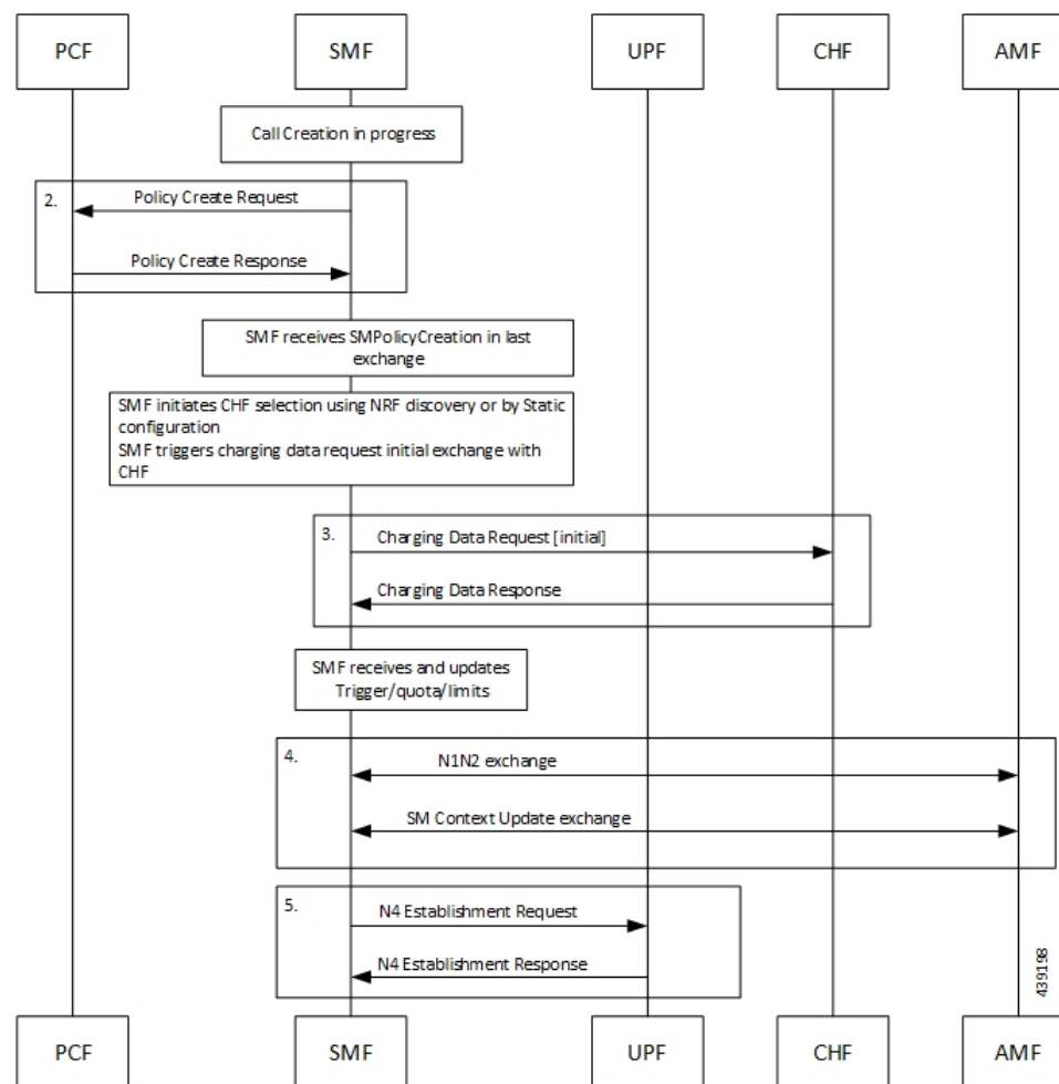
Figure 234: PDU Session Establishment Call Flow
