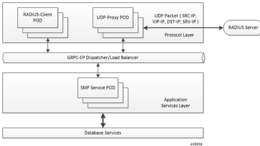
Figure 190: RADIUS Client Integration
