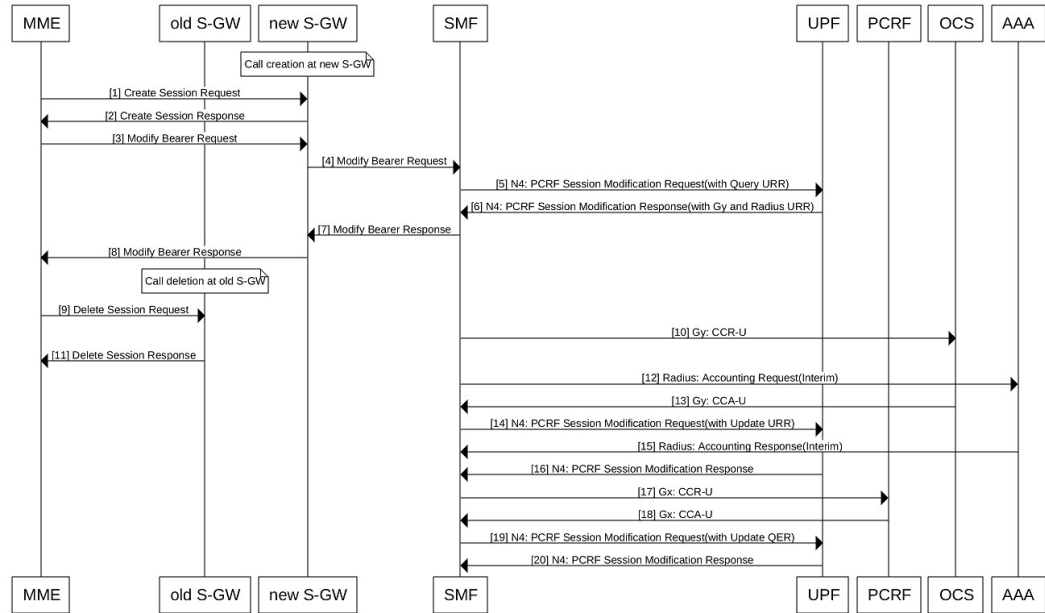
Figure 55: Call Flow for PDN Modification with S-GW Change
