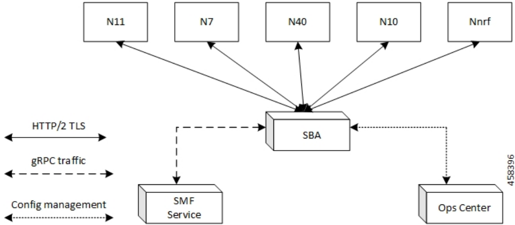
Figure 150: SMF HTTP2 TLS Support for SBA Interfaces
