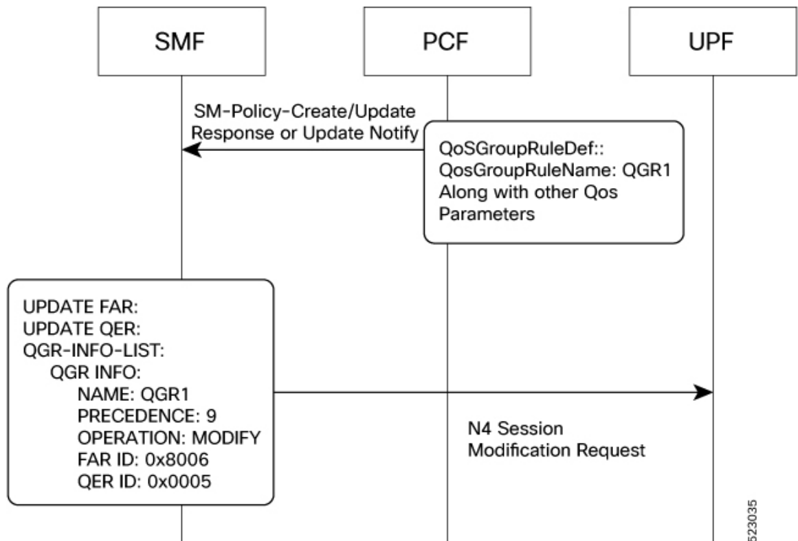
Figure 188: QoS-Group-of-Ruledef Modification Call Flow
