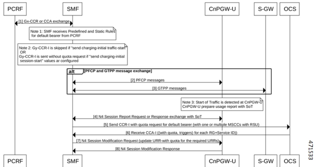
Figure 125: Usage Report with SoT for Predefined and Static Rules
