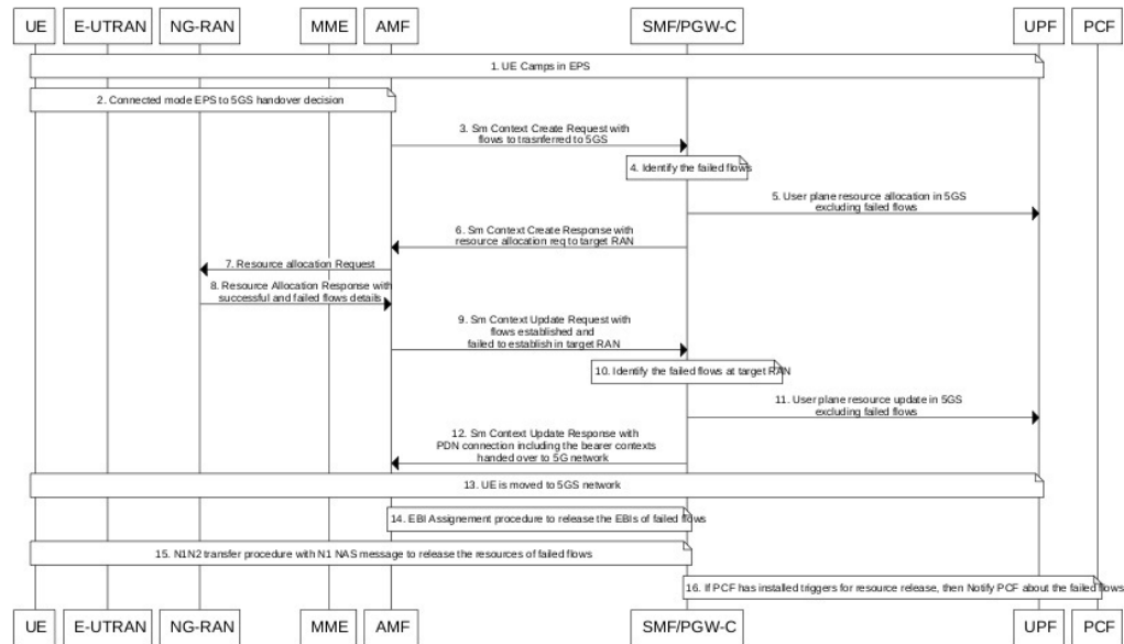
Figure 81: Flow Failure Management Call Flow
