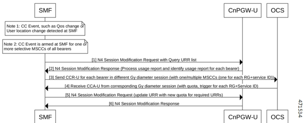
Figure 126: Usage Report in N4 Modify Response (Query URR Scenario)
