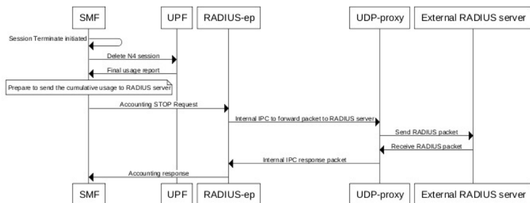
Figure 193: RADIUS Accounting Stop Call Flow
