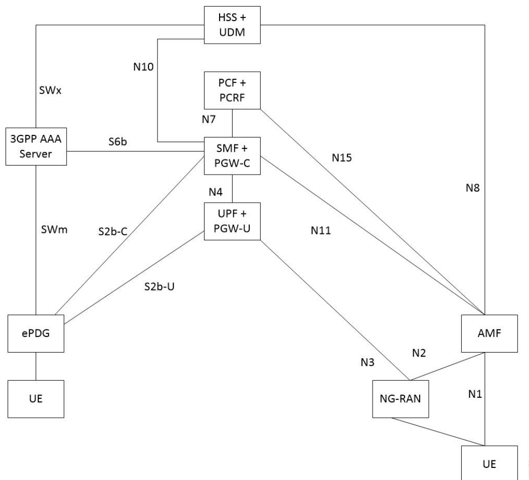
Figure 100: Non-roaming Architecture for Interworking between ePDG or EPC and 5GS
