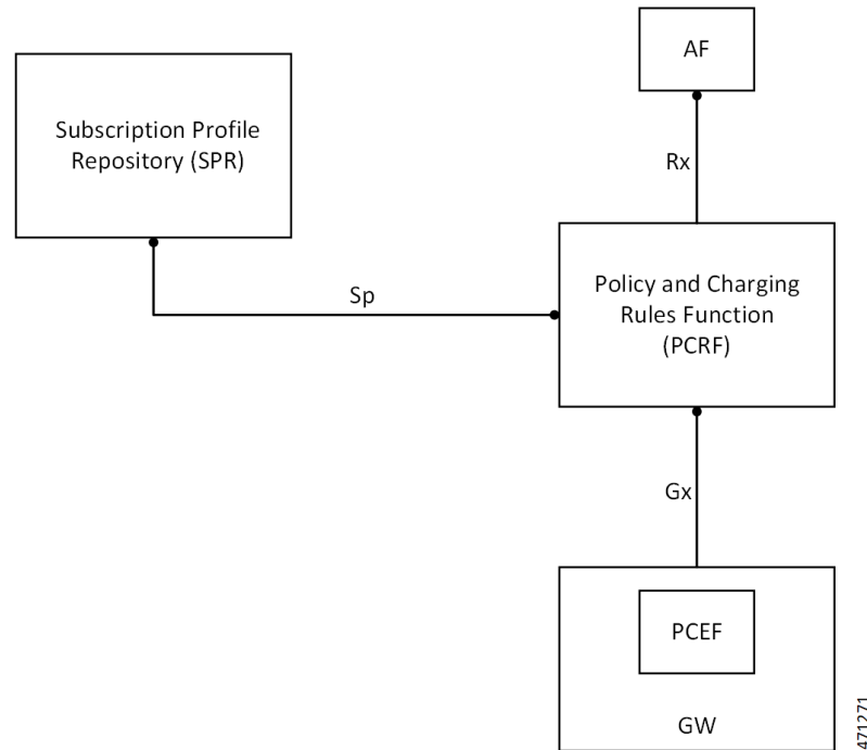
Figure 122: Gx Interface
