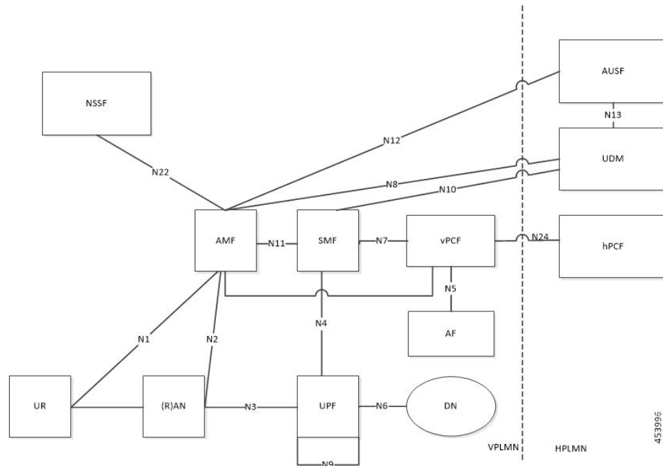
Figure 203: LBO Roaming Architecture for 5G Sessions
