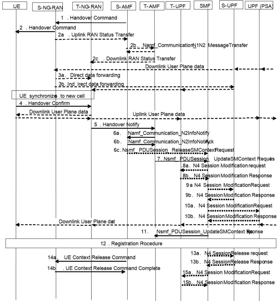
Figure 99: Inter NG-RAN Node N2-based Handover - Execution Phase
