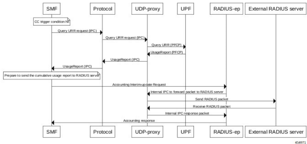
Figure 195: Synchronous Accounting Interim-Update Call Flow
