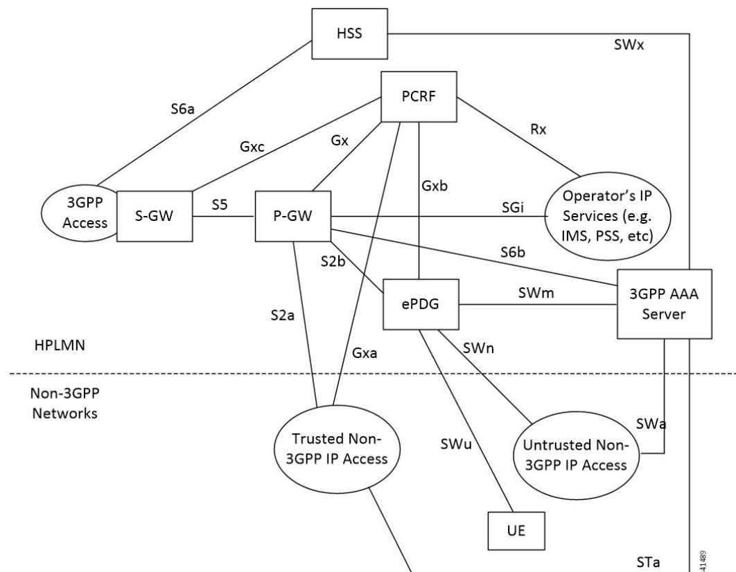
Figure 101: Non-roaming Architecture Within EPS using S5, S2a, and S2b Interfaces
