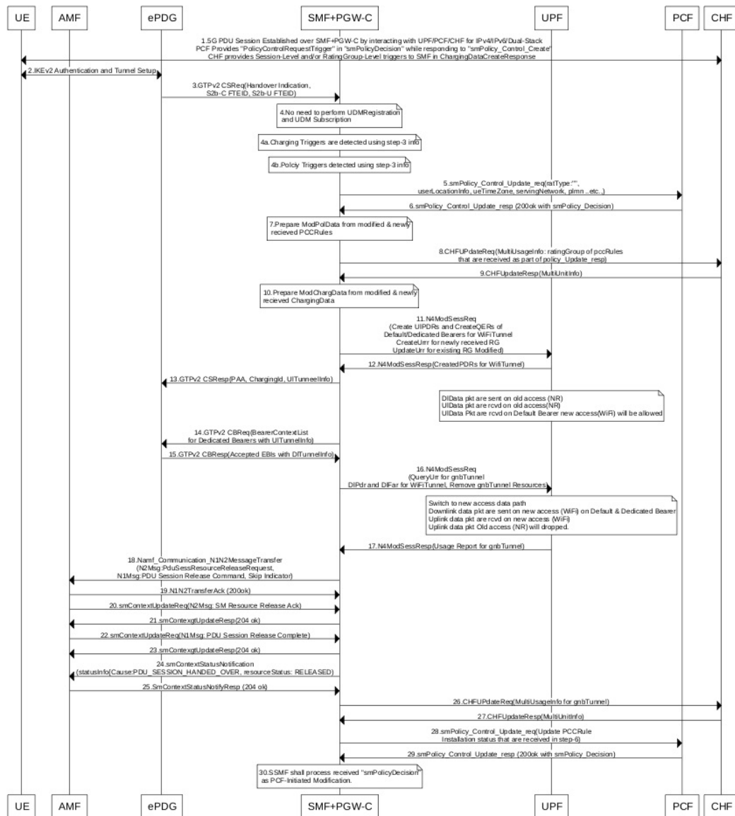
Figure 106: 5GS to Non-3GPP Untrusted Wi-Fi Handover Call Flow
