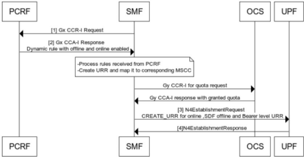
Figure 131: Call Flow
