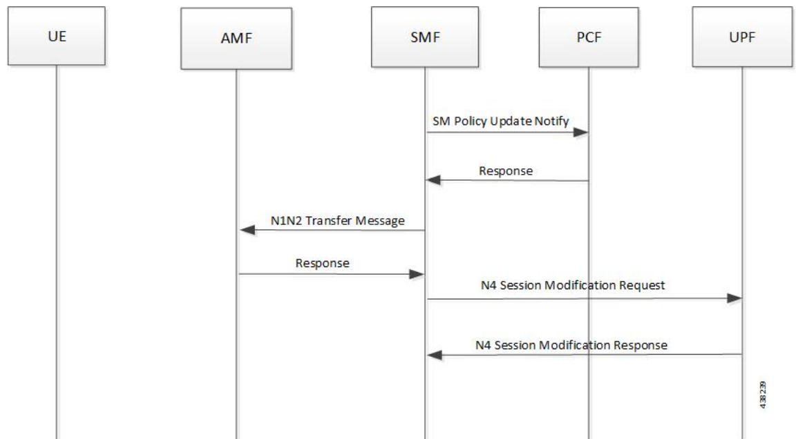
Figure 175: UDM/PCF-initiated Modify
