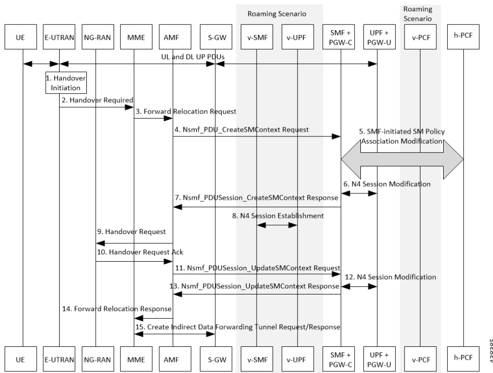
Figure 213: Call Flow for the EPS to 5G Handover Using the N26 Interface
