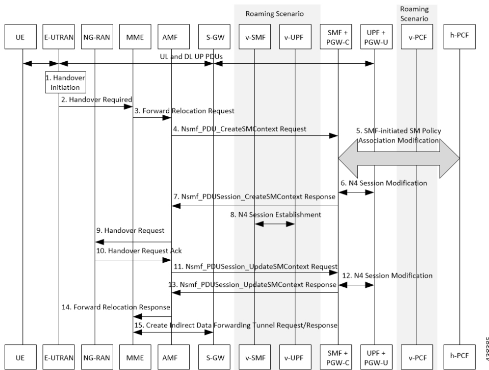
Figure 250: Call Flow for the EPS to 5G Handover Using the N26 Interface
