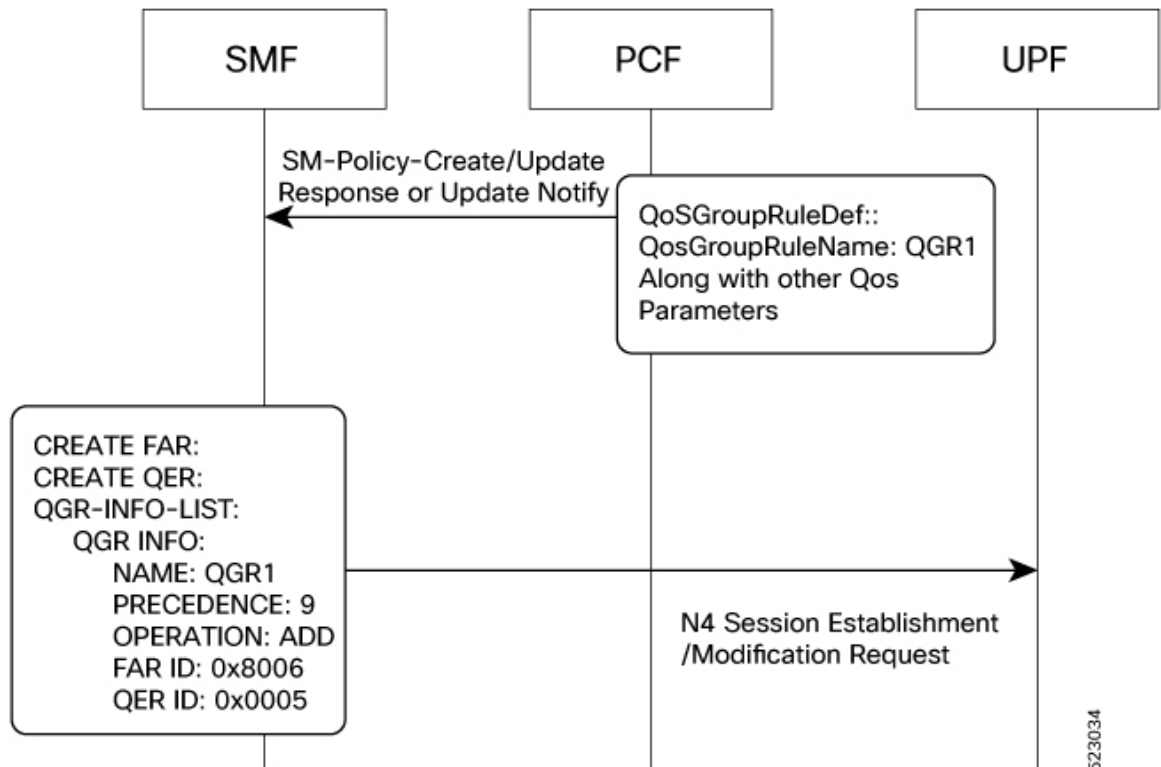
Figure 224: Qos-Group-of-Ruledef Activation Call Flow
