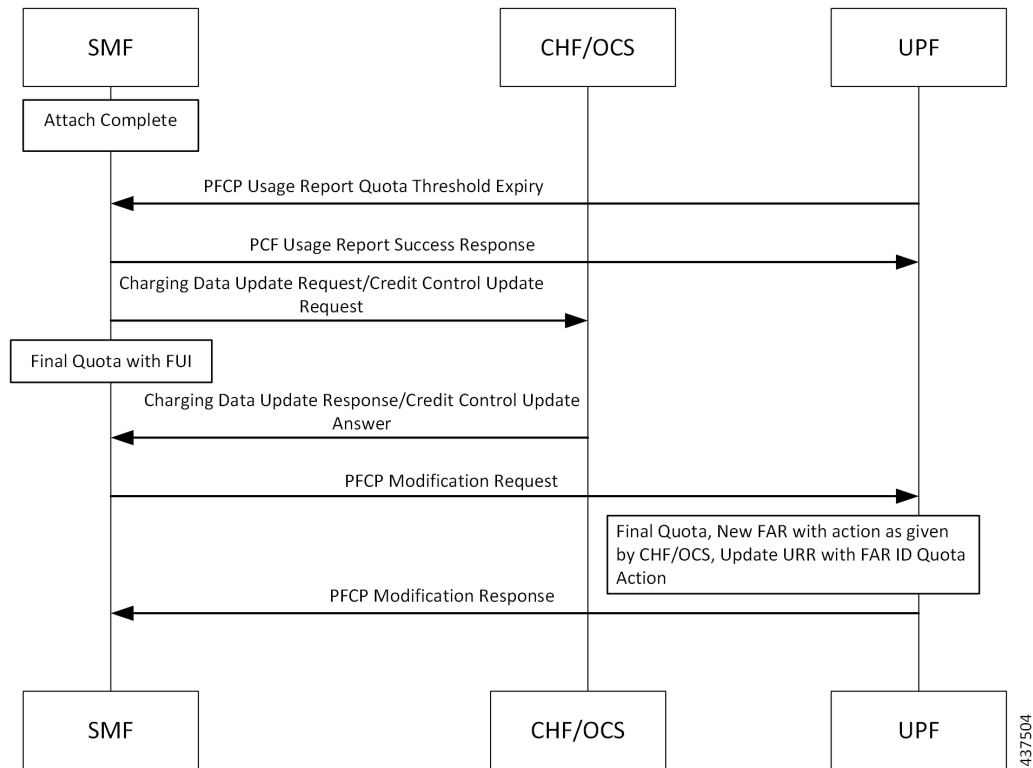
Figure 269: FUI in the Charging Data Initial or Update Response from CHF
