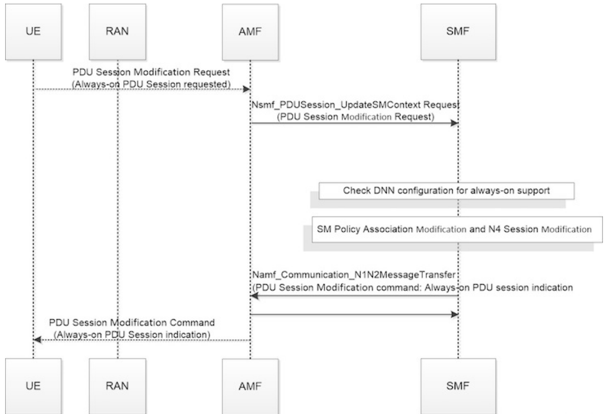
Figure 282: UE-requested PDU Session Modification Call Flow
