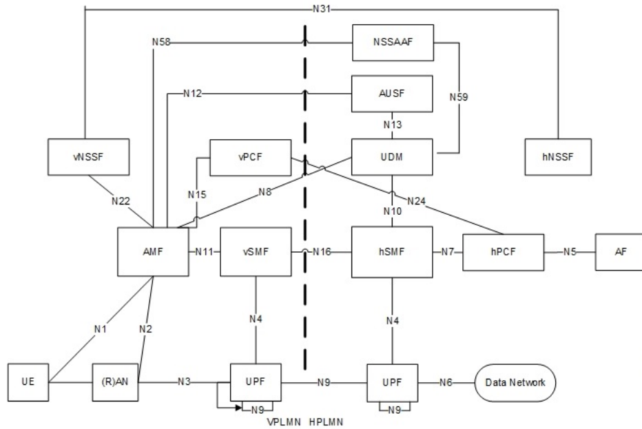
Figure 242: 5G NR HR Roaming Architecture
