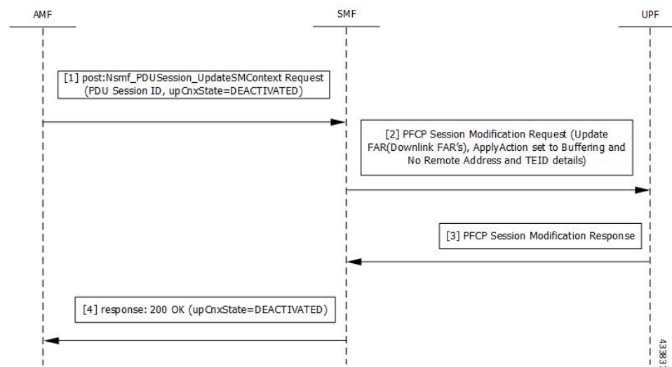
Figure 274: Deactivation of the User Plane Connection Call Flow
