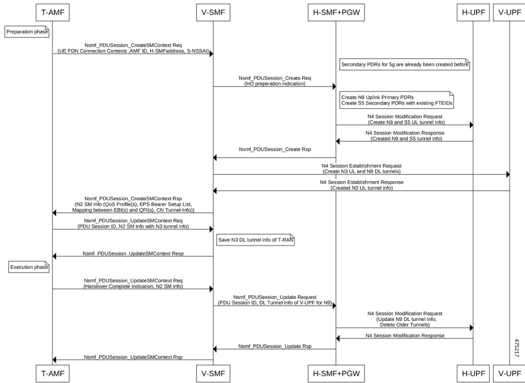
Figure 257: Call Flow for Inter-plmn N26 HO from 4G Homer to 5G Roamer
