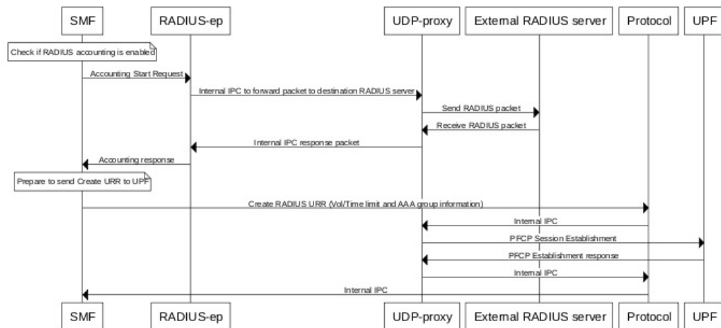
Figure 229: RADIUS Accounting Start Call Flow
