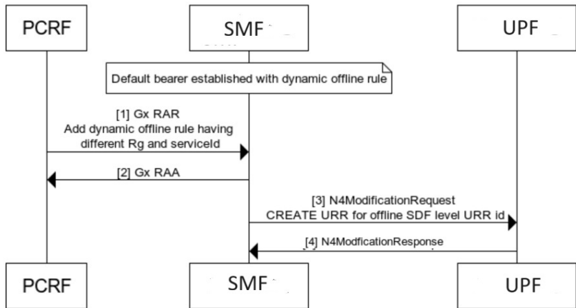
Figure 152: Call Flow for Adding Offline Rules to Default Bearer
