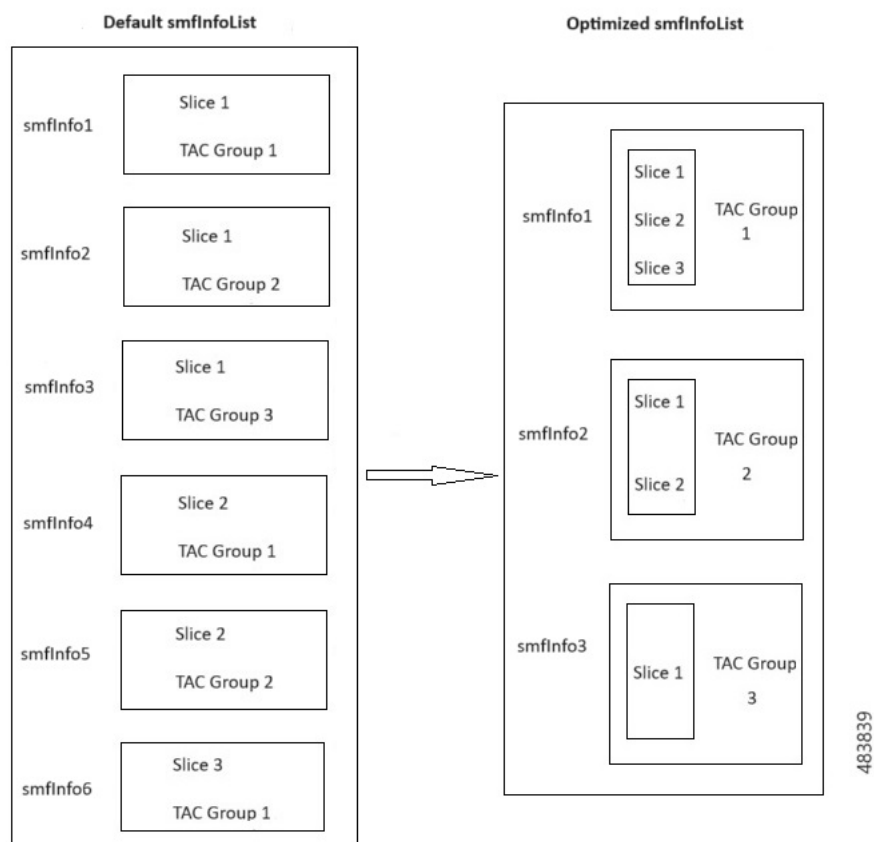
Figure 188: smfInfoList Optimization in NRF Registration Request
