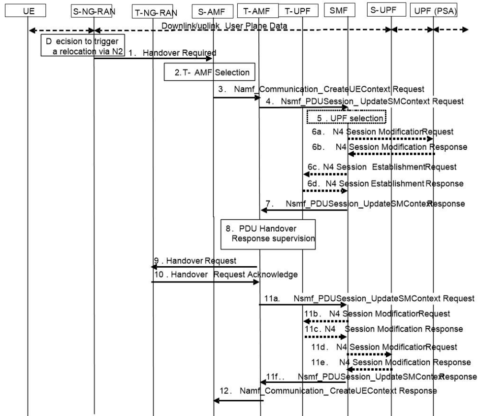
Figure 104: Inter NG-RAN Node N2-based Handover - Preparation Phase
