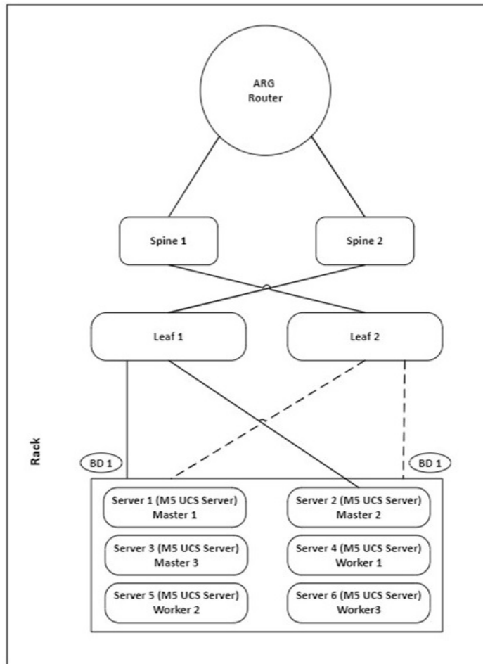
Figure 233: High Availability Layout
