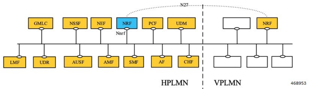
Figure 26: NRF Management
