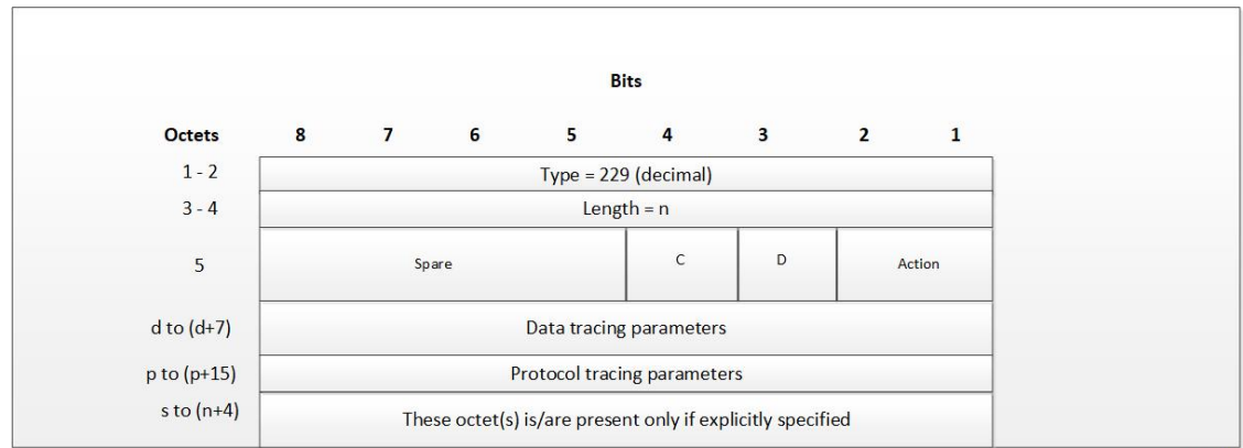
Figure 20: Subscriber Tracing
