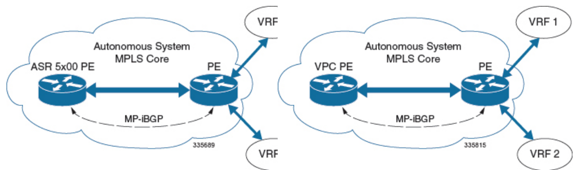
Figure 27: Sample Configuration
