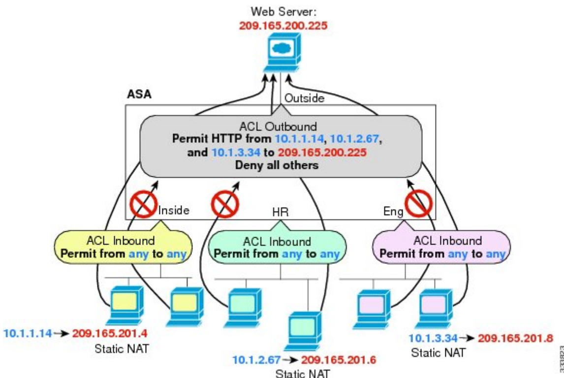
図 2: Outbound ACL
