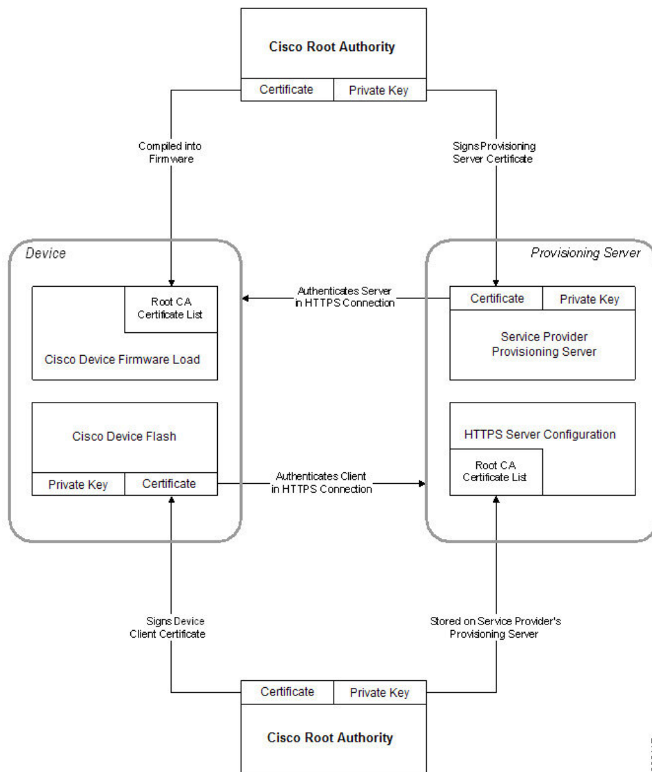
Figuur 7: Certificate Authority-stroom
