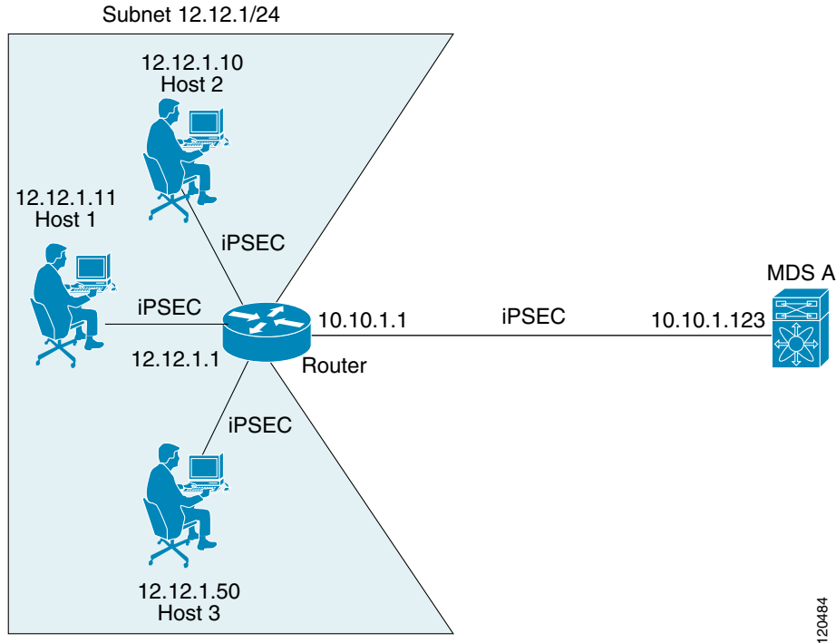
Figure 36-9 iSCSI with End-to-End IPsec
