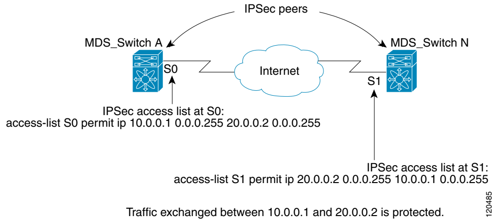
Figure 36-5 IPsec Processing of Crypto IPv4-ACLs
