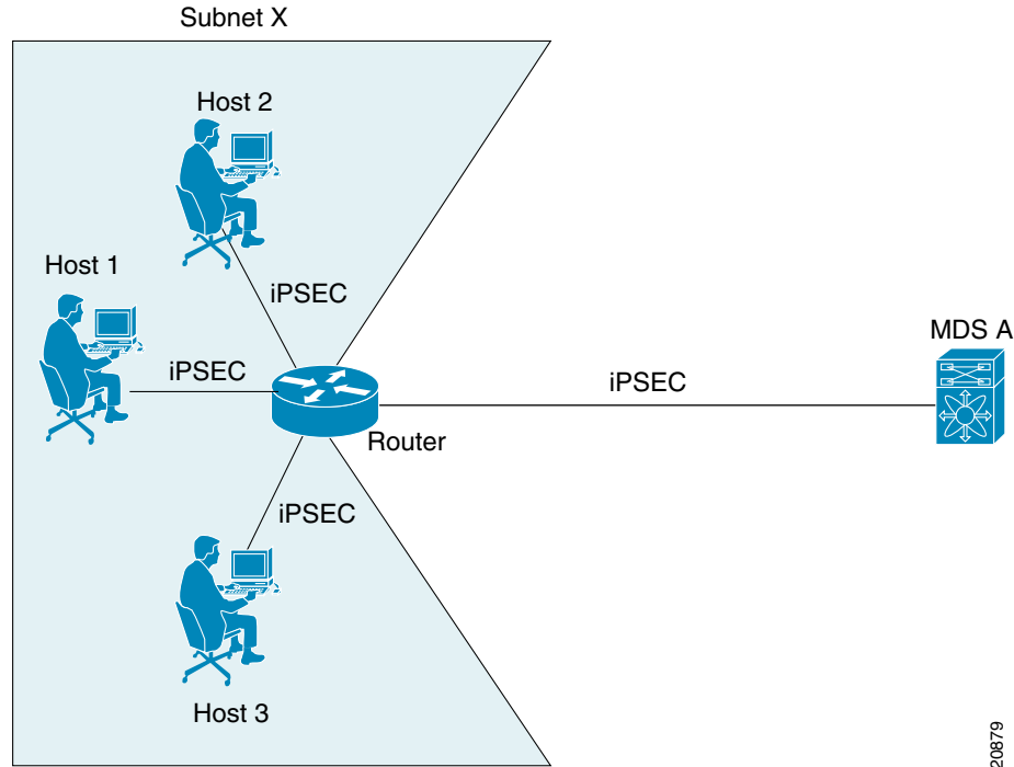
Figure 36-7 iSCSI with End-to-End IPsec Using the auto-peer Option
