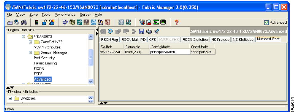
Figure 31-12 Multicast Root Configuration
