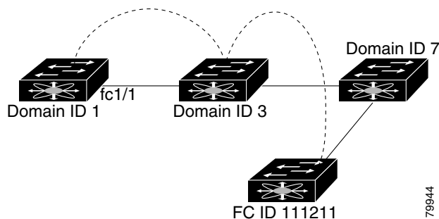
Figure 31-9 Fibre Channel Routes
