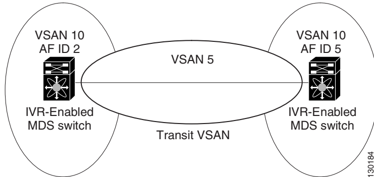
Figure 28-7 Example IVR Topology with Non-Unique VSAN IDs Using AFIDs
