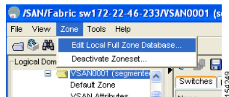
Figure 28-20 Zone Menu
