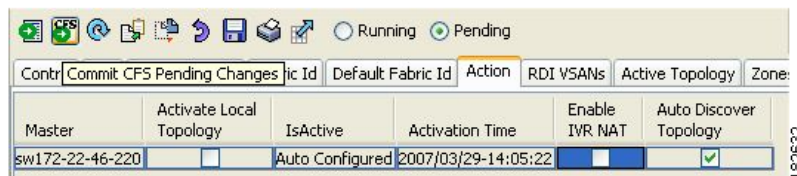
Figure 28-6 Action Tab
