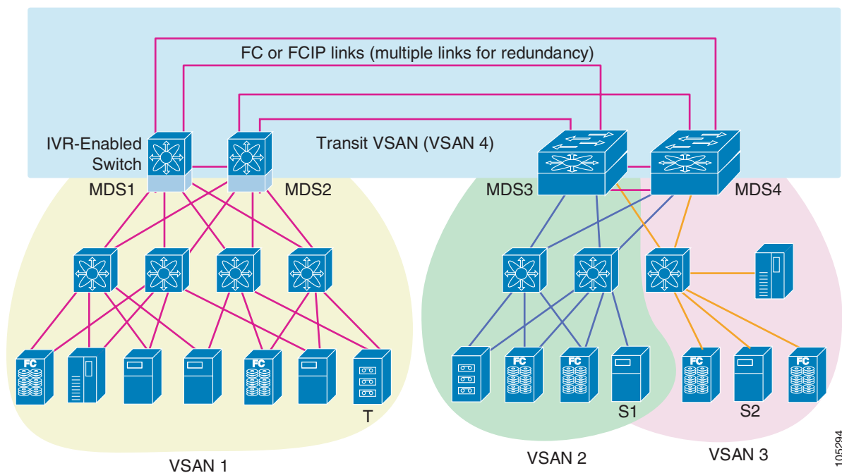
Figure 28-1 Traffic Continuity Using IVR and FCIP
