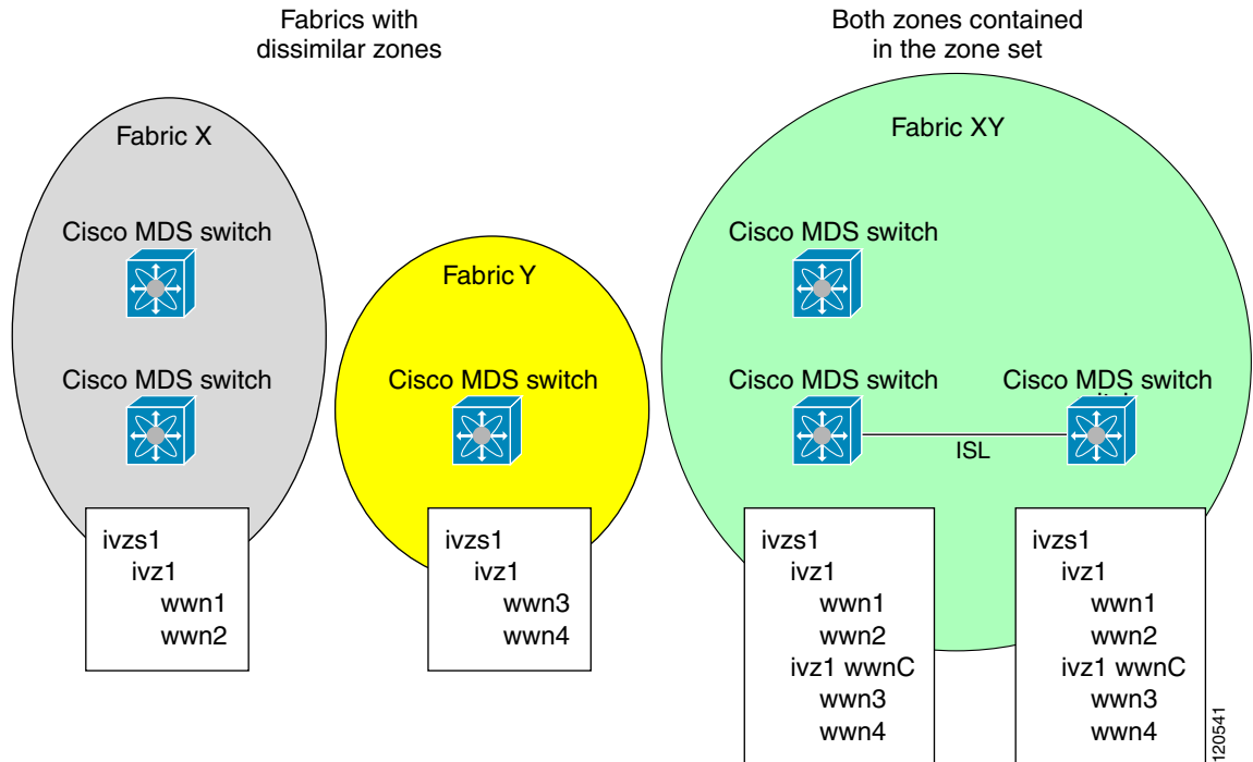
Figure 28-25 Fabric Merge Consequences
