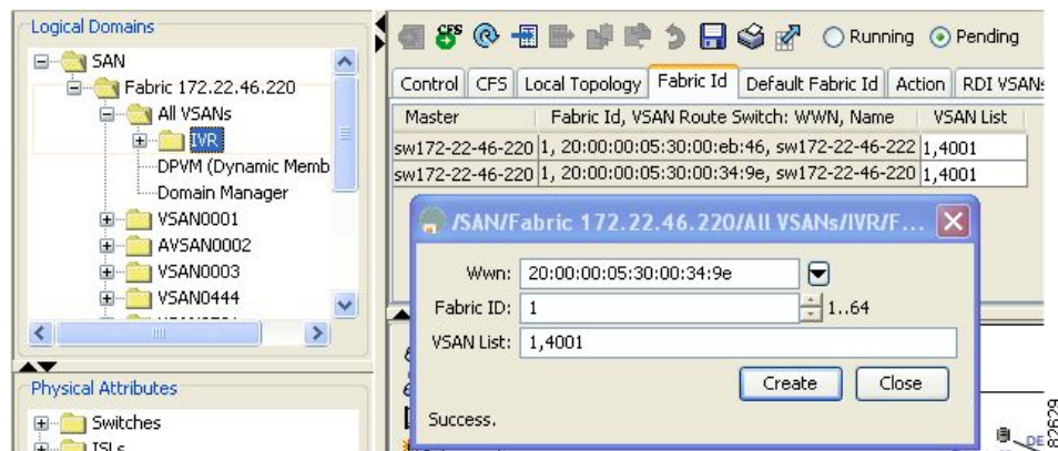
Figure 28-5 Fabric ID Tab
