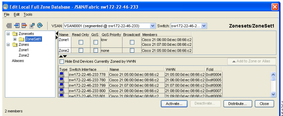
Figure 28-21 Edit Zone Database Dialog Box
