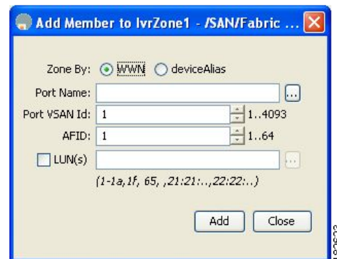
Figure 28-18 Add Member to IVR Zone Dialog Box
