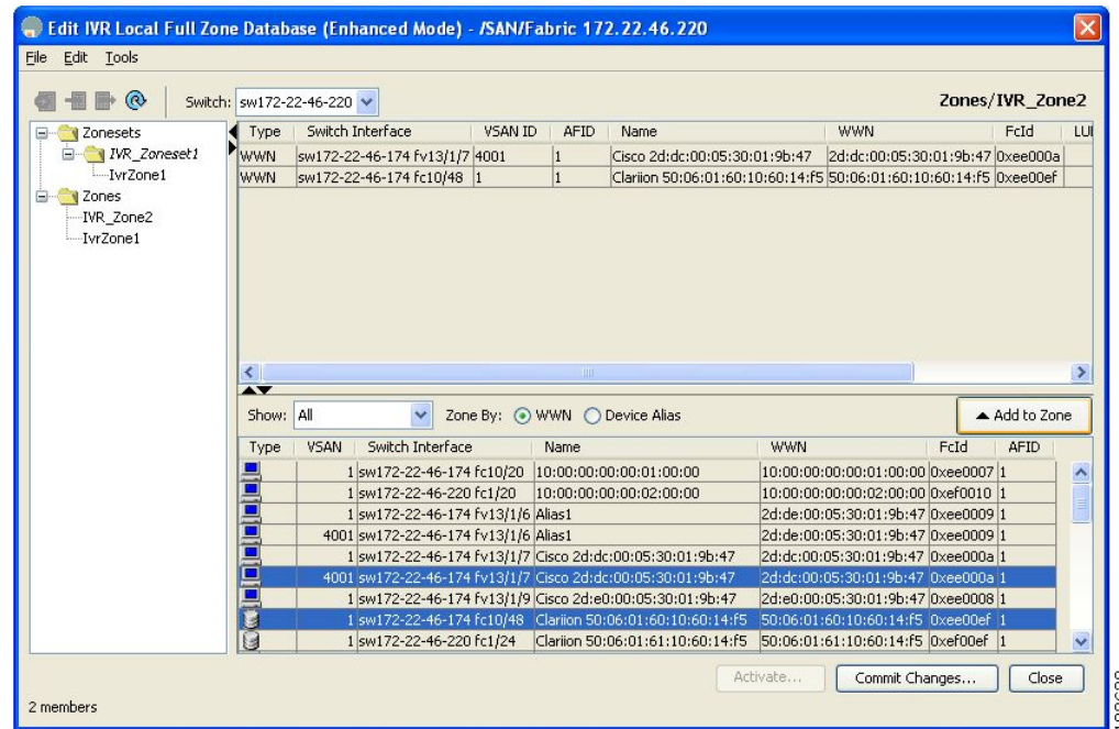
Figure 28-17 Edit IVR Local Full Zone Database Dialog Box
