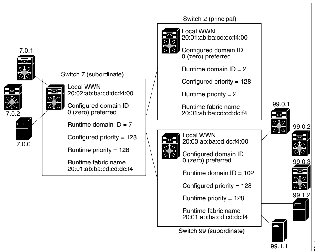
Figure 25-1 Sample fcdomain Configuration
