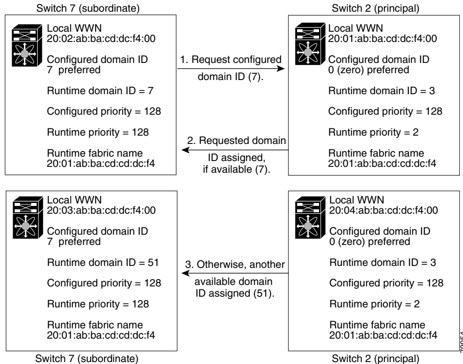
Figure 25-7 Configuration Process Using the preferred Option
