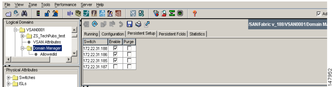
Figure 25-14 Persistent FC ID Information in Fabric Manager
