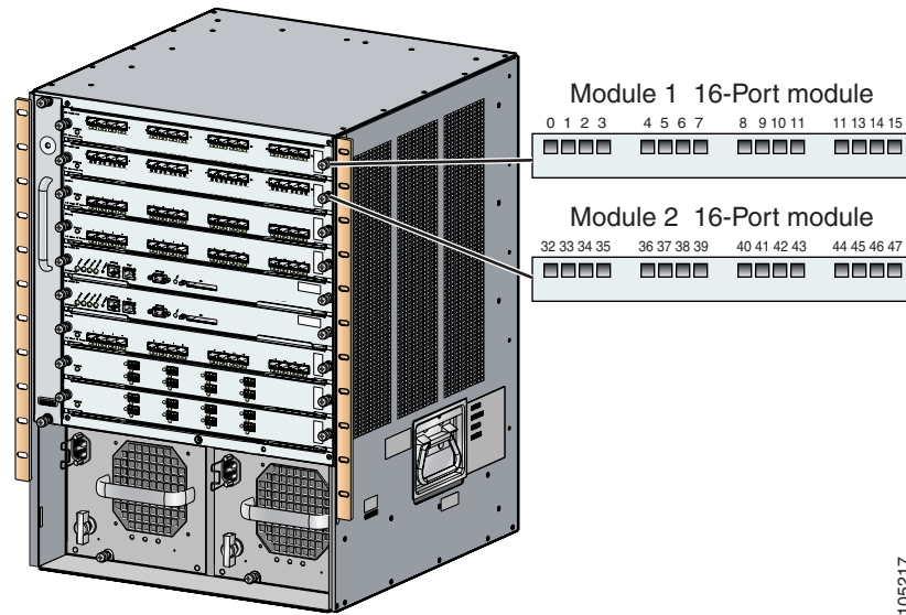
Figure 36-3 Default FICON Port Number in Numbering on the Cisco MDS 9000 Family 9509 Switch
