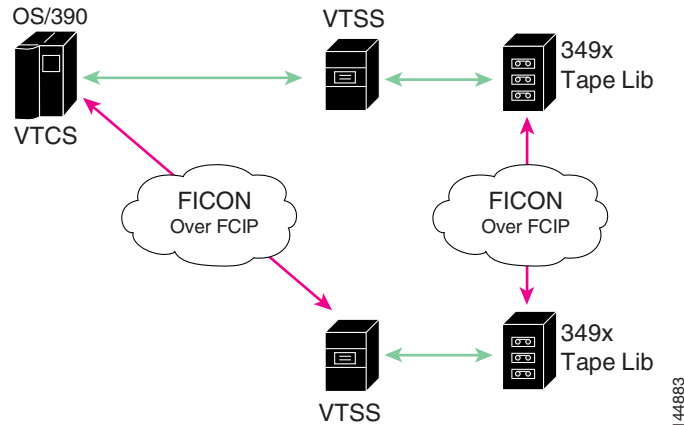
Figure 36-23 Host Accessing Peer-to-Peer VTS (Virtual Tape Server)
